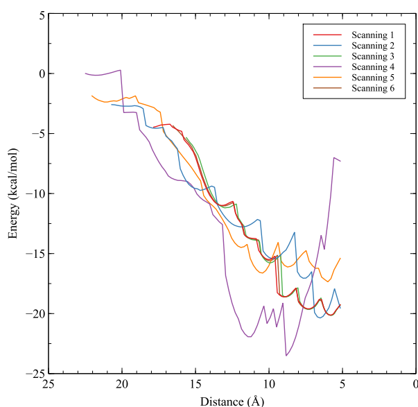
Figure 29. The energy-distance curve of inclusion complex a (Inserting the palmitic acid into the cyclodextrin molecule)
