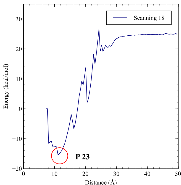
Figure 115 The energy-distance curve of the hexasaccharide-cyclodextrin complex (Removing the cyclodextrin CD#6 from hexasaccharide-cyclodextrin complex)
