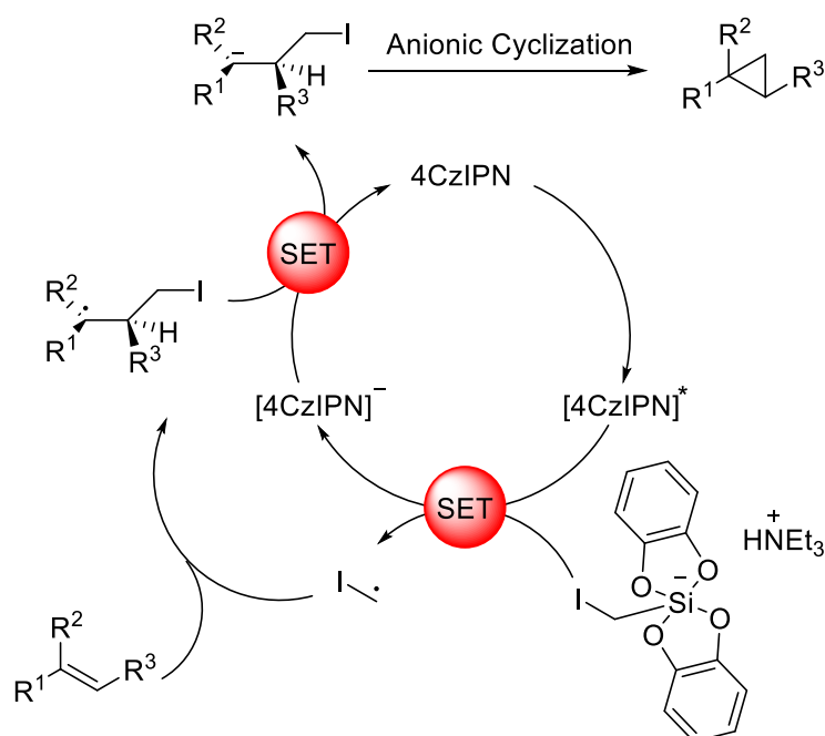
Scheme 87. The proposed mechanism for the cyclopropanation of substituted alkenes with iodomethylsilicates
