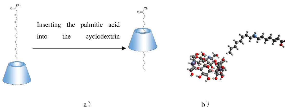
Figure 28. a) Inserting the palmitic acid into the cyclodextrin molecule. b) The starting structure for geometry optimization.
