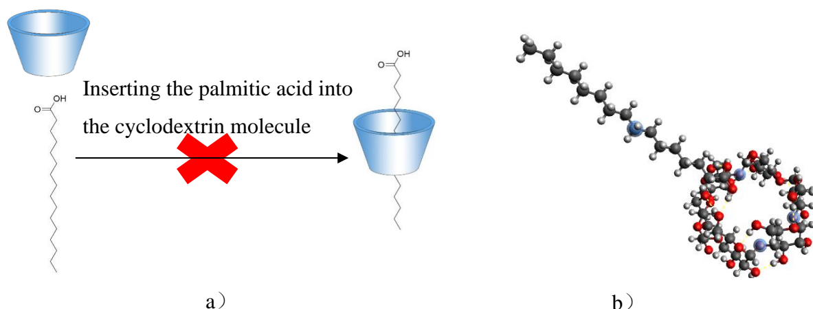
Figure 35. a) inserting the palmitic acid into the cyclodextrin molecule. b) The starting structure for geometry optimization.
