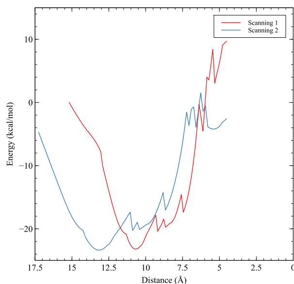
Figure 36. The energy-distance curve of inclusion complex b (Insertion of palmitic acid into the cyclodextrin)
