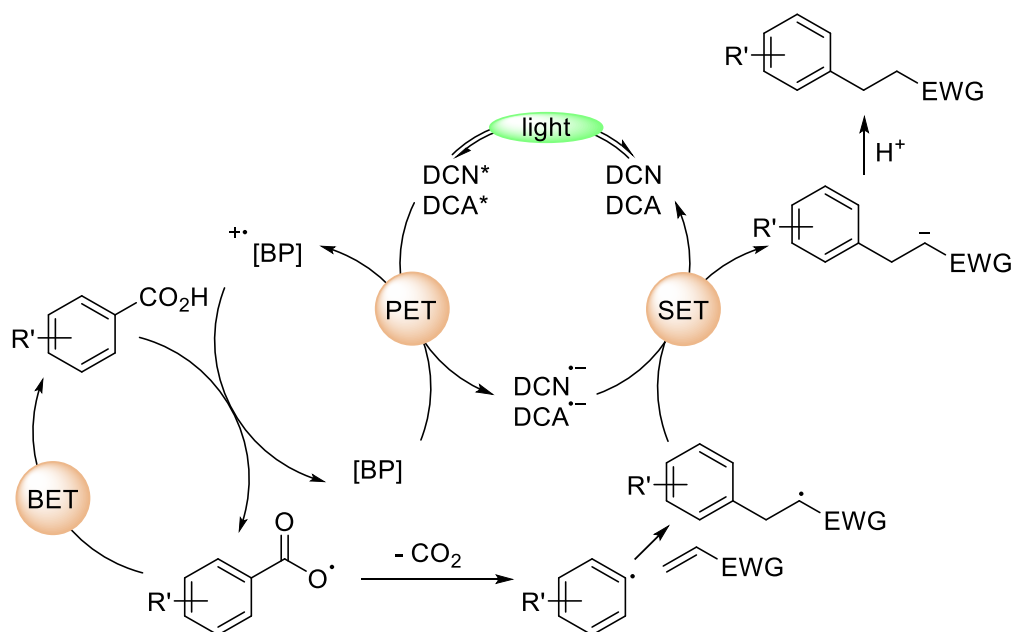
Scheme 46. The proposed mechanism of the photooxidative decarboxylation of benzoic acids via the PET process.
