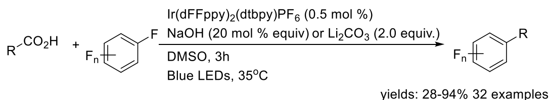
Scheme 47. The photocatalyzed decarboxylative polyfluoroarylation reaction of carboxylic acids
