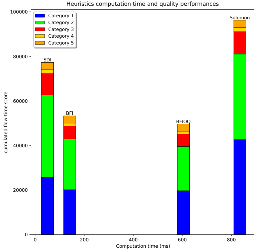
Figure 4.9: Heuristics performances in computation time and objective score
