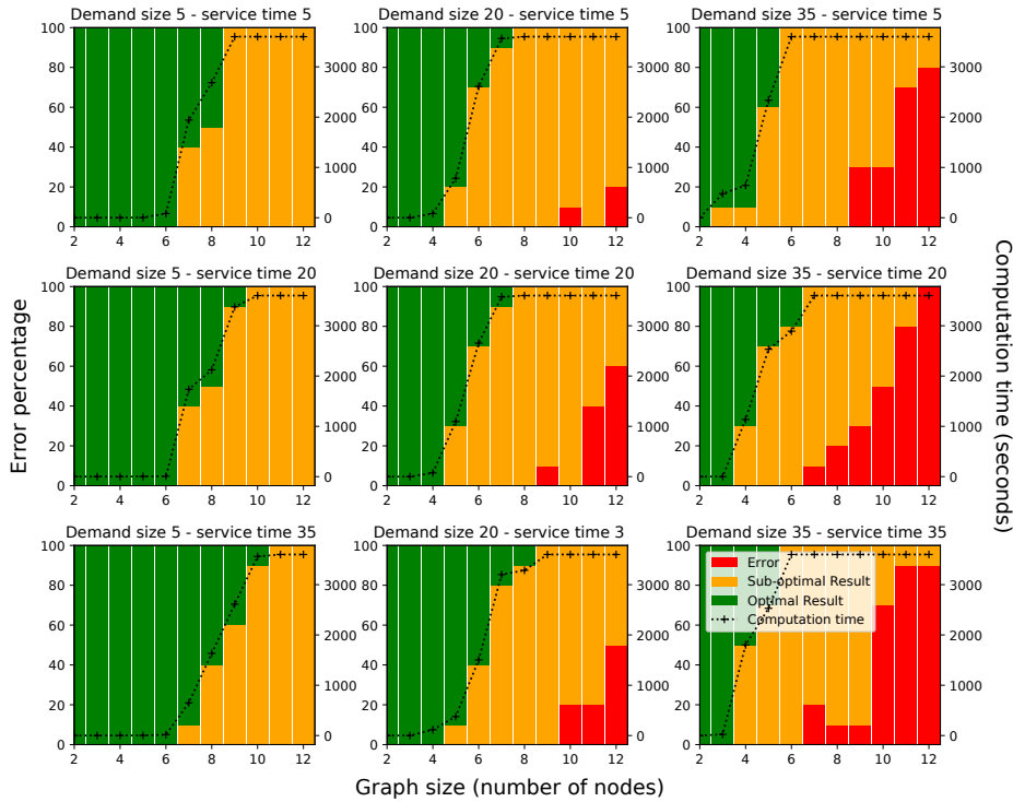
Figure 4.6: Computation time and error rate of MILP according to graph size
