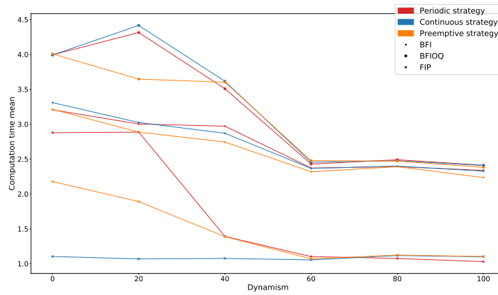
Figure 5.13: Computation time according to dynamism
