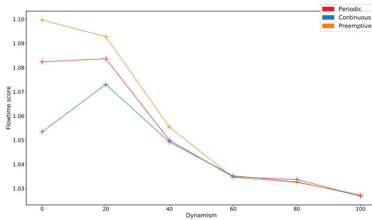
Figure 5.15: Objective score according to dynamism merged by routes computation strategy
