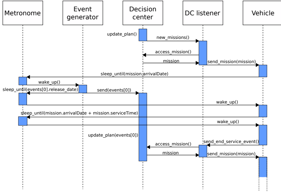
Figure 3.5: Simplified sequence diagram of the simulator
