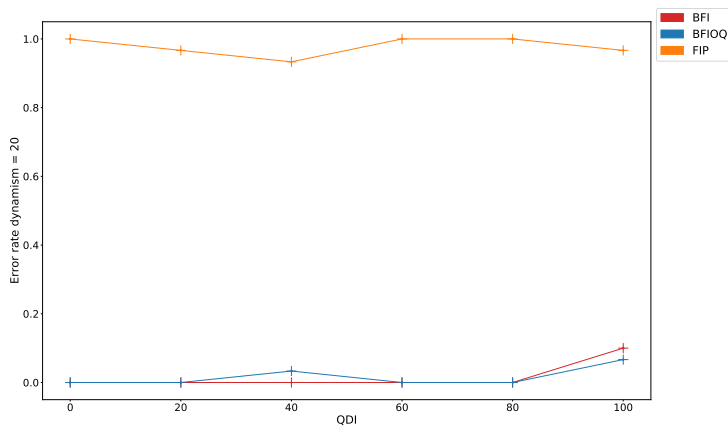
Figure 5.20: Error rate according to QDI dynamism = 20 merged by routes computation heuristic
