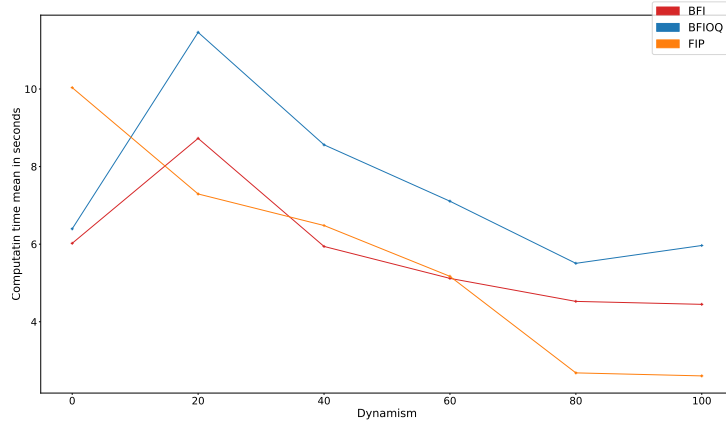
Figure 5.23: Computation time according to dynamism merged by routes computation heuristic
