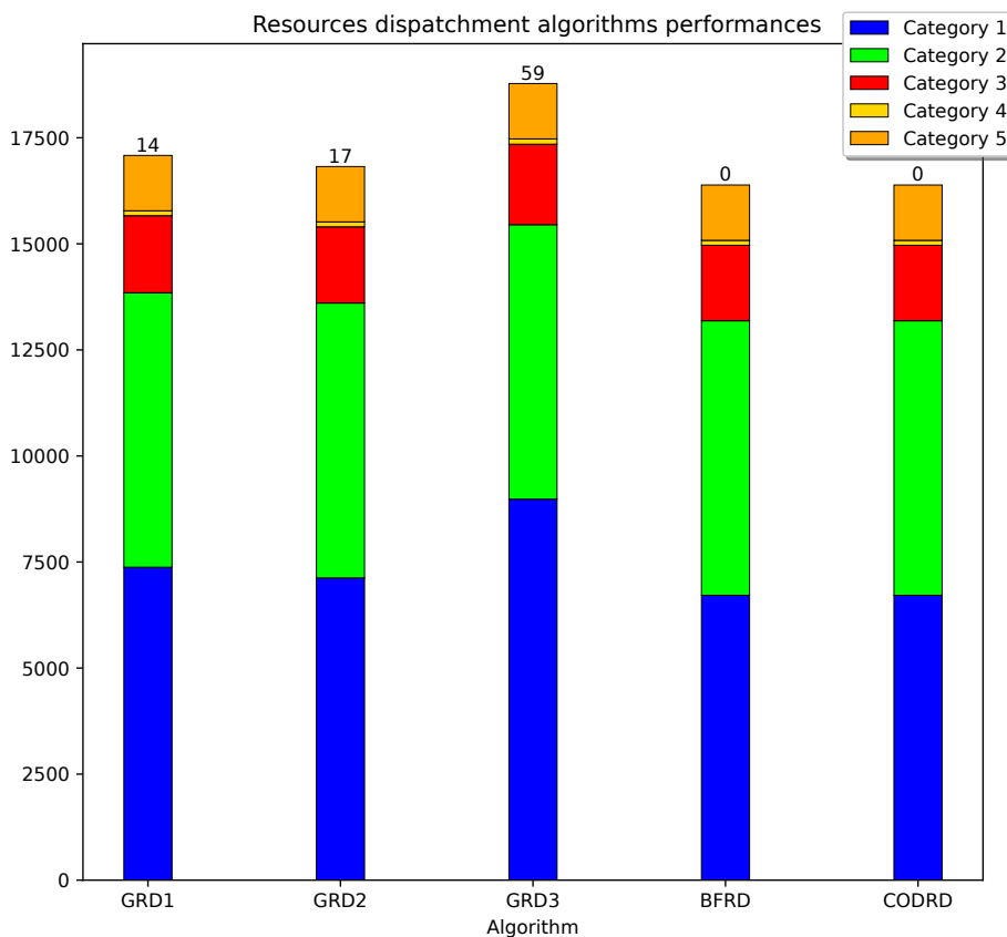
Figure 4.10: Resources distribution solutions evaluation with error percentage in top of the bars
