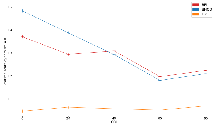
Figure 5.27: Objective score according to QDI merged by routes computation heuristics dynamism = 100
