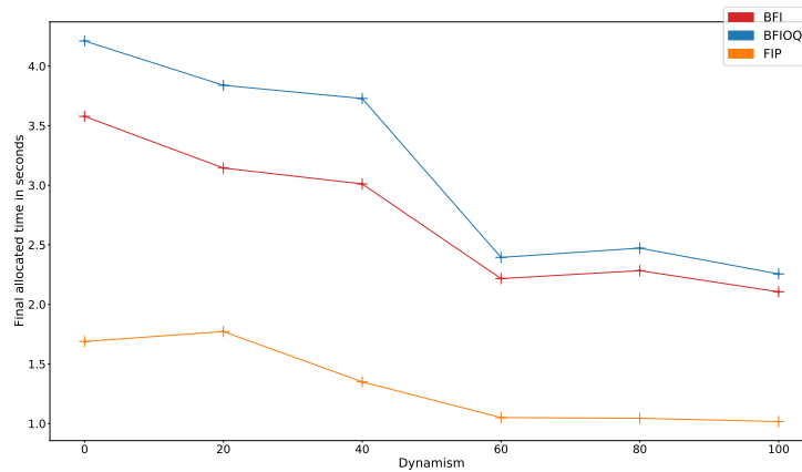
Figure 5.14: Final value of the RCP according to dynamism
