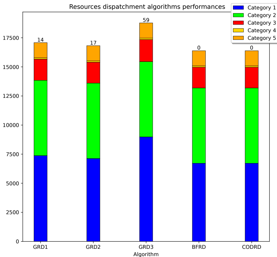
Figure 4.10: Resources distribution solutions evaluation with error percentage in top of the bars
