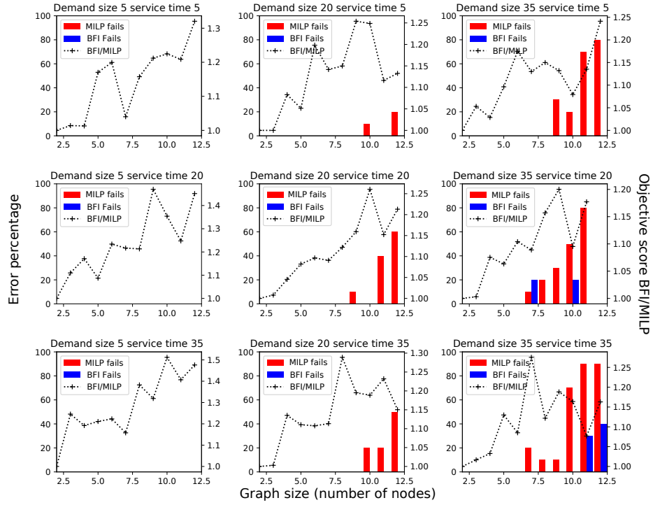
Figure 4.8: Objective BFI/MILP and errors according to problem size
