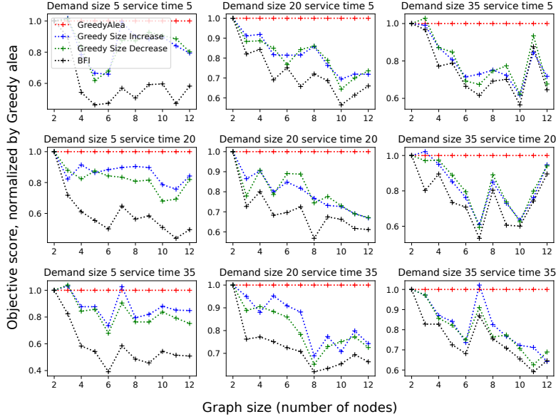
Figure 4.7: Objective score according to graph size of greedy heuristics and BFI
