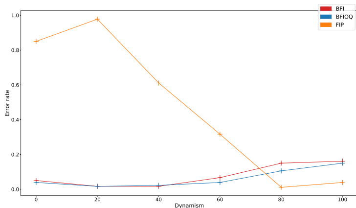
Figure 5.21: Error rate according to dynamism merged by routes computation heuristic
