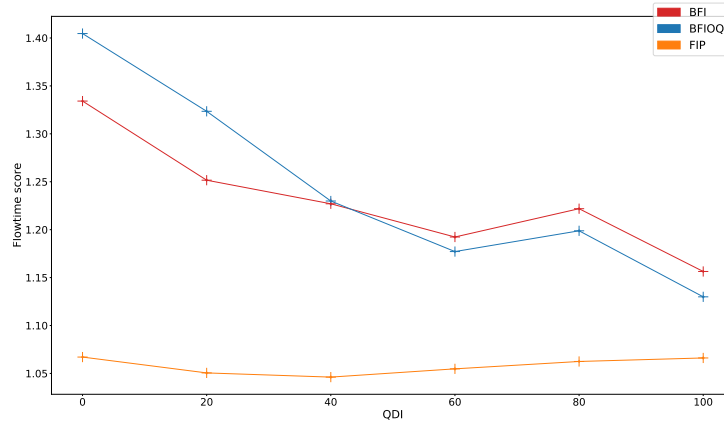
Figure 5.26: Objective score according to QDI merged by routes computation heuristics
