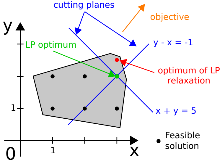
Figure 2.3: Example of step of the cutting plane algorithm
