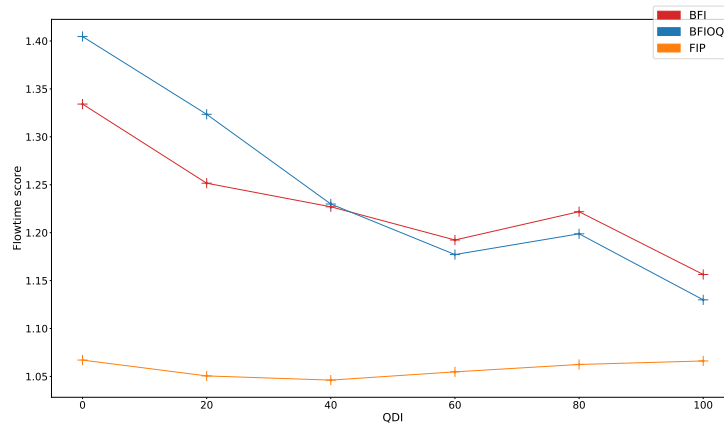
Figure 5.26: Objective score according to QDI merged by routes computation heuristics
