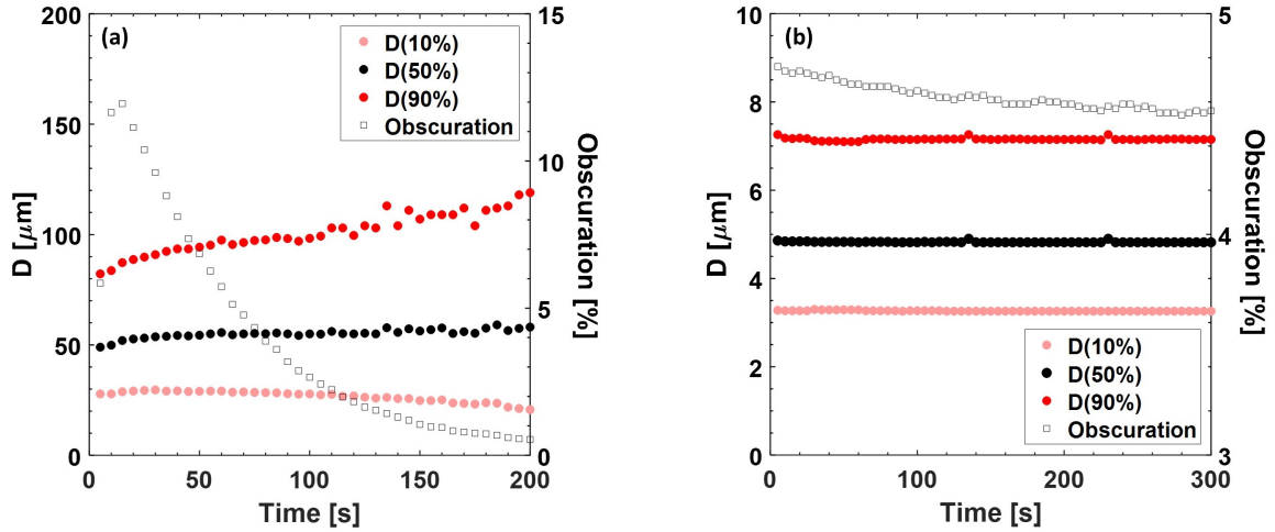
Figure 9.14 – Bubble and drop stability during the measurement. Percentile evolution over time for gas bubbles (a) and oil droplets (b) flowing inside the Mastersizer. The decrease of the obscuration is also reported in both cases. The graphs clearly show the higher stability of droplets.
