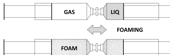
Figure 6.1 – Double-syringe method. Two syringes partly filled with air and foaming solution are connected, and foaming occurs by pushing both fluids repeatedly through the constriction given by the syringe inlets.
