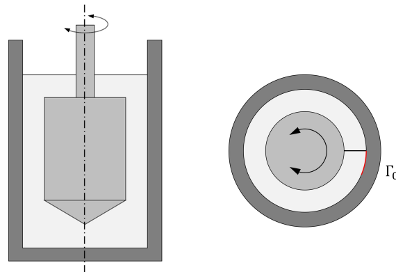
Figure 7.1 – Cylindrical Couette geometry. Vertical (left) and horizontal (right) section of the cylindrical Couette geometry used for emulsion rheology measurements. The rotating inner cylinder applies a sinusoidal strain with increasing amplitude \Gamma_0 to the emulsion inside the stationary cup.
