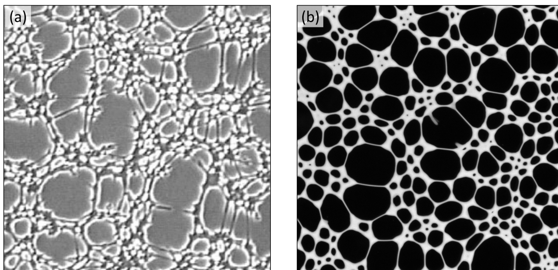
Figure 7.24 – Morphology comparison. (a) Mixture of polystyrene and diethyl malonate undergoing viscoelastic phase separation after thermal quenching, seen under a phase-contrast microscope. The edge size is 556 \mu\text{m} . Picture taken from [115]. (b) Emulsion distribution at late stage of coarsening in a foamed emulsion at \phi = 80\% . The edge length is 7 cm. The resemblance with the phase-separating polymer mixture is remarkable.
