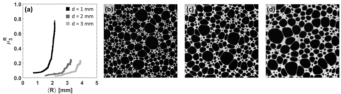
Figure 7.29 – Bubble pattern at different cell spacing. (a) Third moment of the radii distribution \mu_3^R vs the average bubble size \langle R \rangle . The larger the gap d , the larger the critical bubble size at which \mu_3^R steeply increases, reflecting the onset of the delayed disappearance of small bubbles. (b,c,d) Photos at the end of the image acquisition at gap equal to 1, 2, and 3 mm respectively. The edge size of the pictures is 12 cm.
