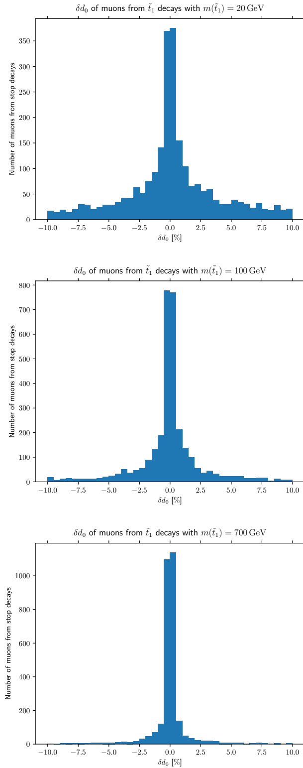
Figure 5.5: Relative difference \delta d_0 between the exact and approximate formulæ of d_0 for muons originating from the decay of the selected long-lived R -hadrons for samples of three different stop masses.
