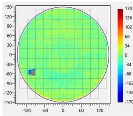
FIGURE 2.19 – Focus spot
