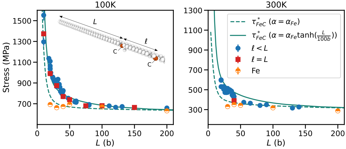
Figure 4.9: Dependence of the average unpinning stress on the largest dislocation segment length L . MD at (a) 100 K and (b) 300 K. Blue circles are when \ell < L , red squares when \ell = L . Half-filled orange symbols refer to the flow stress in pure iron computed by MD in cells of different lengths L . The dashed and solid lines are predictions of a statistical model (see text for details).
