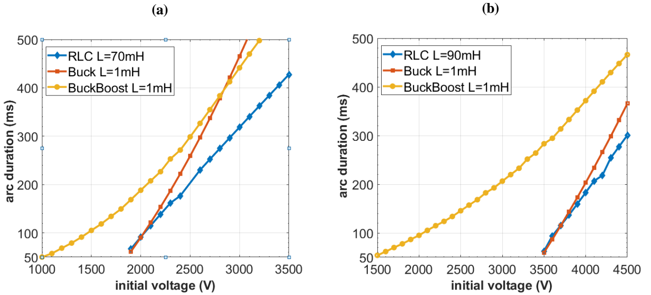
FIG. II.10 Comparison of the performances of RLC, Buck and Buck-boost circuits considering a load resistance of 4 Ω (a) and 8 Ω (b).
