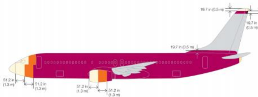
FIG. I.9 Lightning zone applied to a Boeing airliner – overview (a) and sideview (b) (Sweers et al. (2012)).
