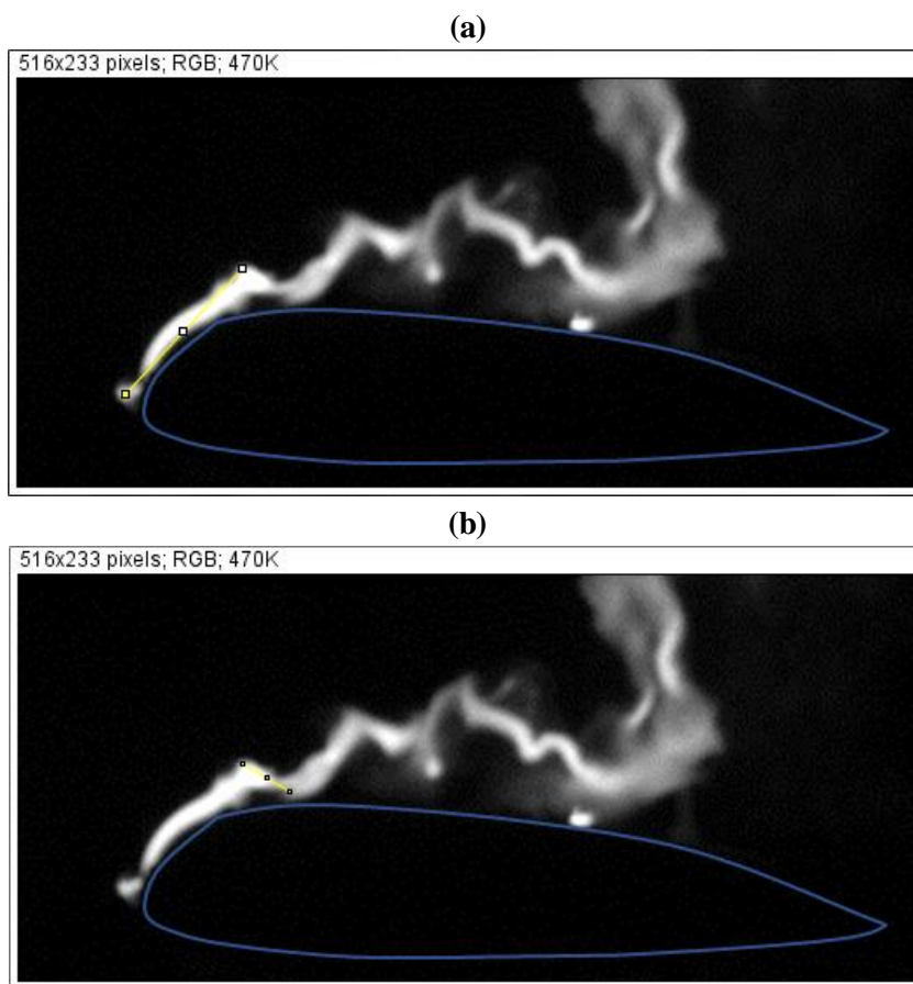
FIG. V.8 Two consecutive image adjustments of arc channel length before extinction and reattachment. The yellow lines are adjusted to the different arc column straight portions and their lengths are added to give a measure of the extinguished arc channel portion.
