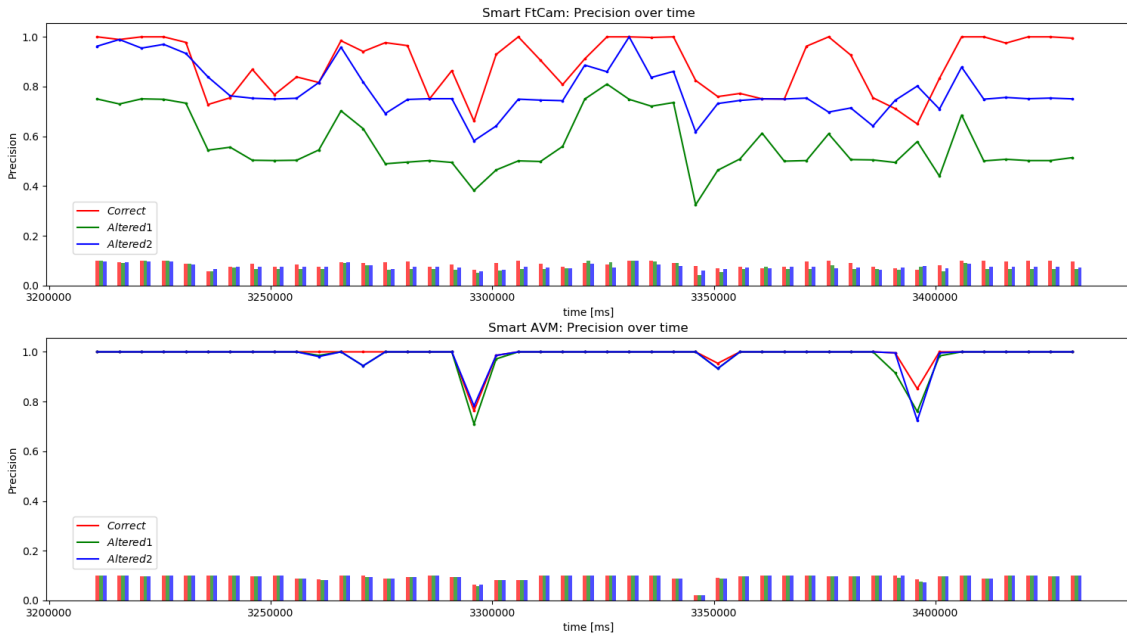
Figure 4.10: In the case of Smart FrontCam, Precision results generally higher for Correct , which makes possible its distinction from Altered1 and Altered2 . On the other hand, all of the N_l recordings report similar trends from the standpoint of the Smart AVM.
