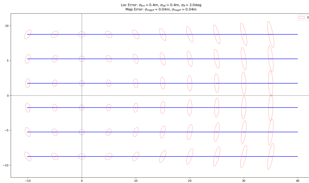
Figure 4.4: Position uncertainty ellipses for localization error of heading \sigma_{\theta}=3^{\circ}
