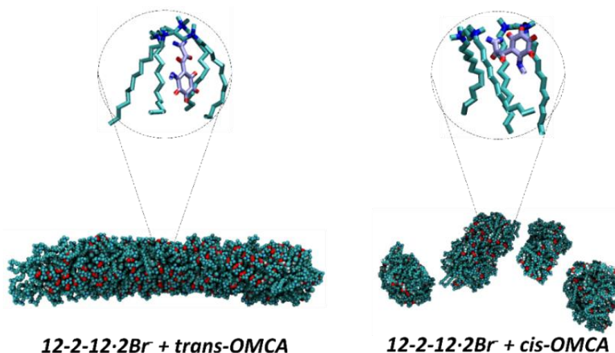
Fig. 2.7 The arrangements of 12-2-12·2Br - and OMCA molecules on micelles at r_n = 0.75 . (The cyan parts are 12-2-12 2+ ; the red parts are OMCA - ; the red beads and white beads are oxygen atoms and hydrogen atoms in OMCA.)
