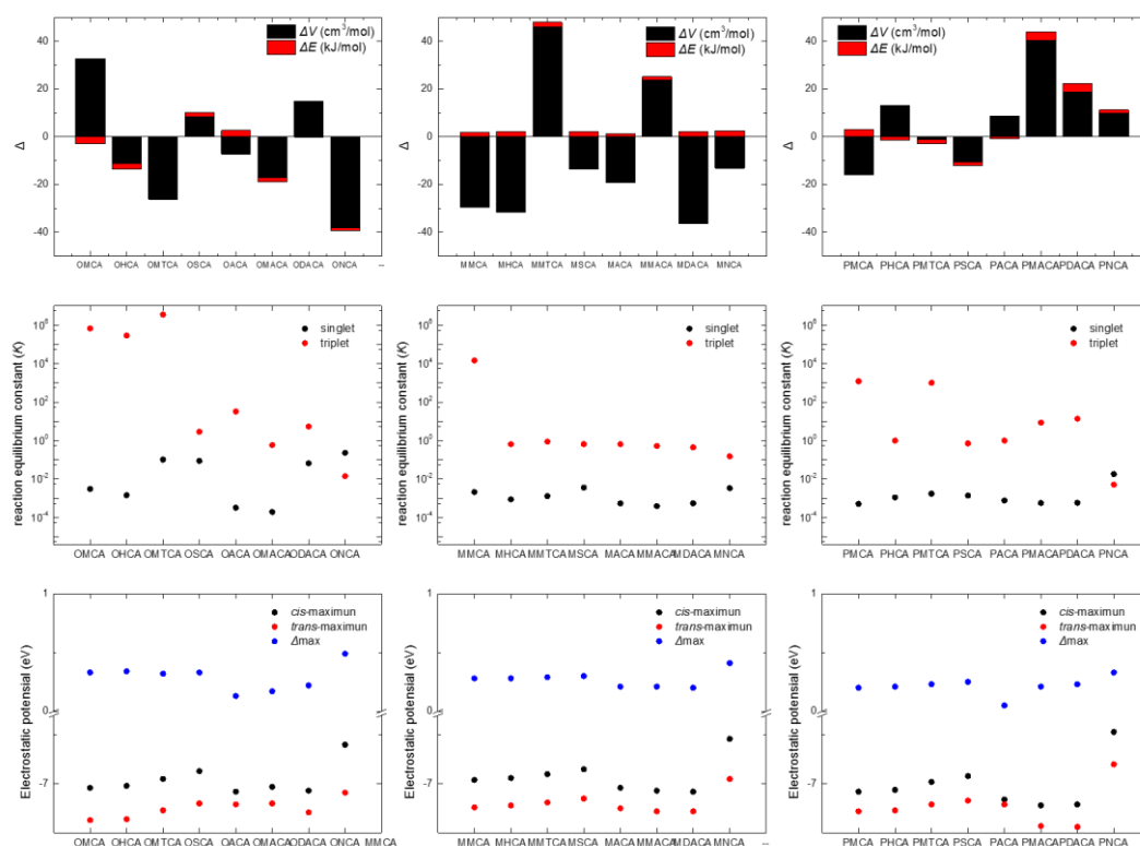
Fig. 4.14 The calculated difference of ionic molar volume ( \Delta V ( \text{cm}^3/\text{mol} ) the black column) and solvation free energy ( \Delta E ( \text{kJ/mol} ) the red column), and photo-isomerization reaction equilibrium constants at singlet state K_{g-s} and triplet state K_{g-t} , the maximum of negative electrostatic potential (eV) cis -maximun, trans -maximun, and their difference \Delta_{\max} of trans/cis -cinnamic acids after UV irradiation.
