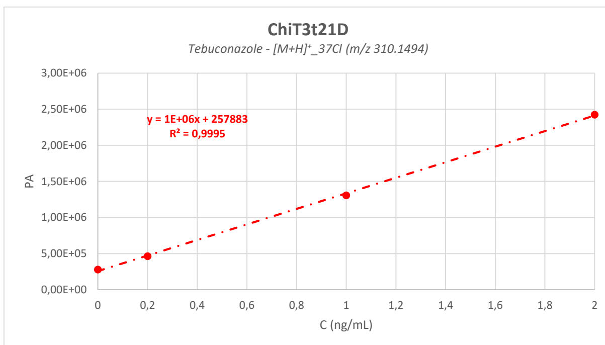
Figure S11. Calibration curves of standard addition traced for each standard in each sample integrating the area of the [M+H]^+_{35Cl} ion and comparing with the [M+H]^+_{37Cl} . 5 standards were added: Boscalid, Pyraclostrobin, Fenbuconazole, Fluopyram and Tebuconazole. 3 repetitions of “Ctr” contaminated untreated controls samples and 3 repetitions of “Chi” treated samples were used for this experiment.
