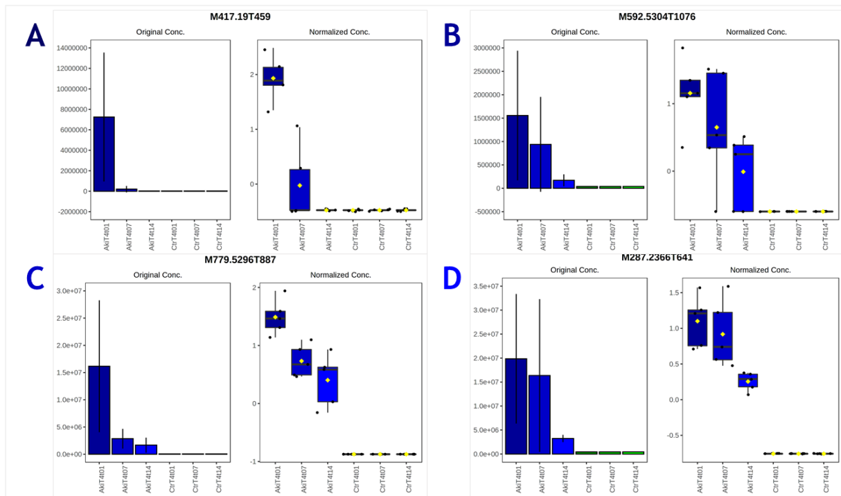
Figure S4. Boxplots of the 4 Akivi xenometabolites features representing the 4 different degradation kinetics patterns (A, B, C, D) identified on the heatmap ( Fig. 2 ).
