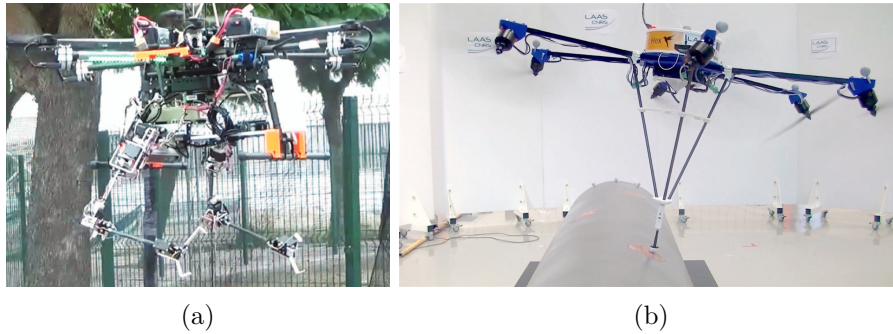
Figure 1.4: Second generation of aerial manipulators: (a) An aerial dual-arm manipulator with compliant joints [Ollero 2018]; (b) A fully actuated platform interacting with the environment [Ryll 2019]
