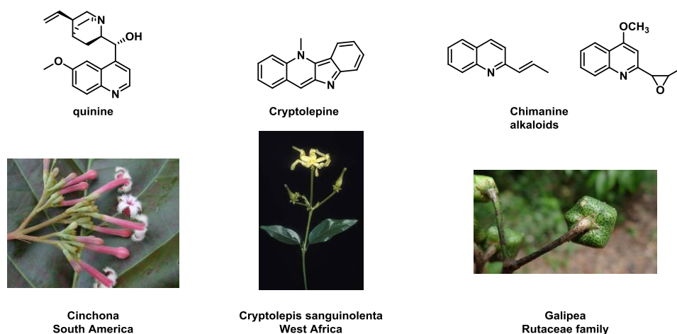
Figure 54: Natural alkaloids
