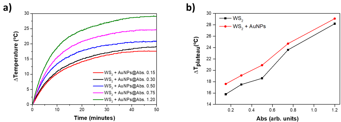
Figure 6-18 : a) Photothermal response of WS_2/Au hybrid materials with different absorbance ( viz. concentration). b) Comparison of the photothermal response between pristine WS_2 and hybrid WS_2/Au as a function of different absorbance ( viz. concentration).
