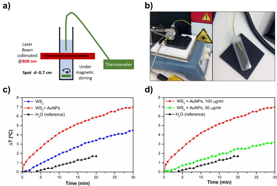
Figure 6-17 : a) Sketch and b) images of the experimental set-up used for the photothermal analysis. c) Photothermal response of pristine WS_2 and hybrid WS_2/Au compared to water, possessing both a concentration of 100 \mu g/ml . d) Photothermal response of hybrid WS_2/Au systems with different concentration.
