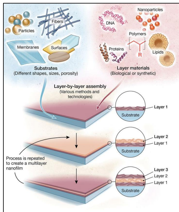
Figure 1.1 A schematic view of layer-by-layer assembly [2].
