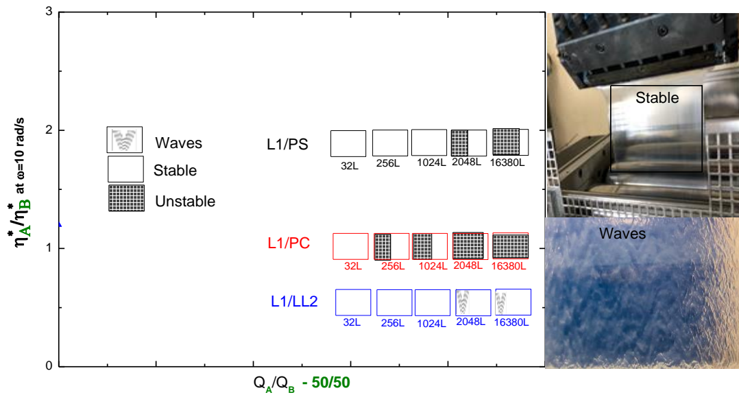
Figure 4.1 Chart of stability/instability observed experimentally for different couples of coextruded films with the plot of viscosity ratios at \omega=10 rad/s versus composition using a reference temperature of 240^\circ\text{C} .
