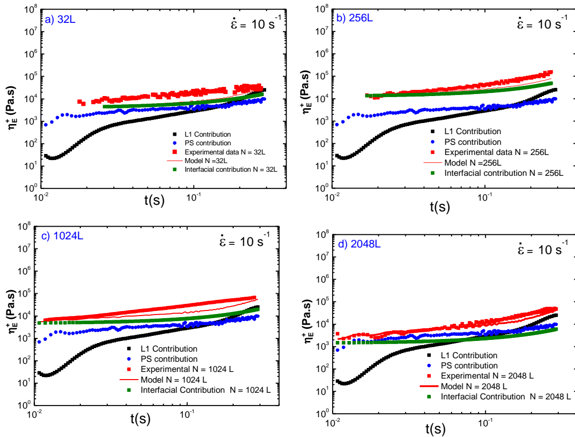
Figure 3.22 Contributions from L1 layers, PS layers, and interface summed to show the multilayer tensile stress growth coefficient predicted Eq. (55) overlaid with experimental data at 10 \text{ s}^{-1} .
