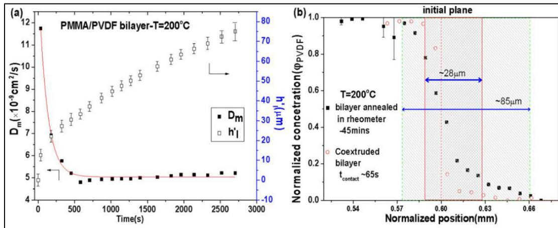
Figure 1.13 (a) Time evolution of the mutual diffusion coefficient and interphase thickness of a PMMA/PVDF bilayer heated at 200^\circ\text{C} : (b) Normalized PVDF concentration profile versus normalized position determined from SEM-EDX in the cross-section of the bilayer after being heated for 45 min (solid black squares) and the coextruded bilayer (open red circles). [43].
