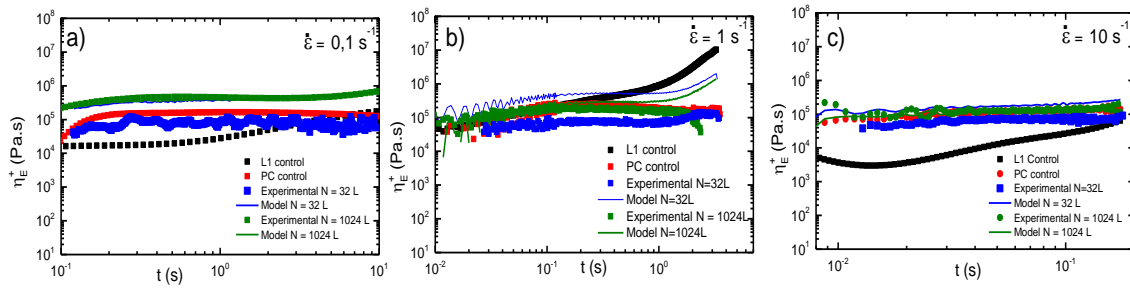
Figure 3.25 Tensile stress growth coefficients of LDPE-L1 (black squares) and PS (red circles) homopolymers, in addition to LDPE-L1/PS 32 layer and 1024 layer films coupled with solid lines representing model fitting at (a) 0.1 \text{ s}^{-1} , (b) 1 \text{ s}^{-1} , and (c) 10 \text{ s}^{-1} strain rates.
