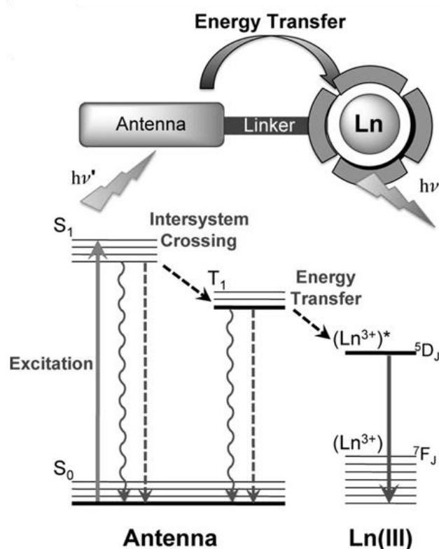
Figure 1.4. ( Top ) The general architecture of an emissive Ln(III) ion chelated and linked with an antenna for absorbing excitation; ( bottom ) a simplified Jablonsky diagram illustrating antenna effect.
