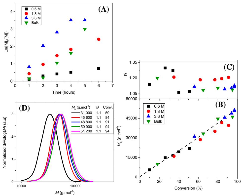
Figure 3.4. Kinetics of the RAFT polymerization of terpene acrylate at 80 °C in toluene at various monomer concentrations (Squares) [M]_0 = 0.6 mol.L -1 ; (Circles) [M]_0 = 1.8 mol.L -1 ; (Up triangles) [M]_0 = 3.6 mol.L -1 ; (Down triangles) bulk (entries 9-12 in Table 3.3). The DP_n = [M]_0/[DBTTC]_0 ratio is kept at DP_n = 250 . (A) Evolution of the \ln([M]_0/[M]) as a function of time. (B) Evolution of the measured molar masses as a function of monomer conversions; the dash line is a guide for the eye. (C) Evolution of the dispersity values as a function of monomer conversion. (D) Molar mass distributions (from SEC-MALS) of poly(terpene acrylate) prepared by RAFT polymerization at 80 °C ( [M]_0 = 3.6 mol.L -1 , DP_n = 250 ) at various monomer conversions.
