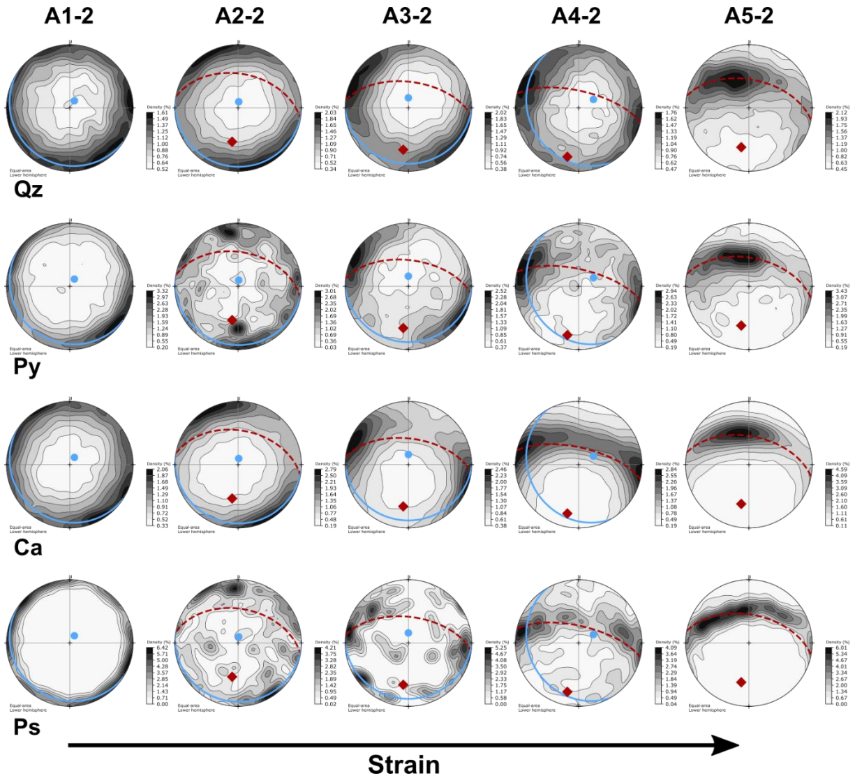
Figure 4.16: Stereoplots of ellipsoids' long axes ( L_1 ) for quartz, pyrite, calcite and pores in the five samples (A1-2 to A5-2). Here the pole of bedding (blue) and cleavage (red) are the mean poles measured in the field.
