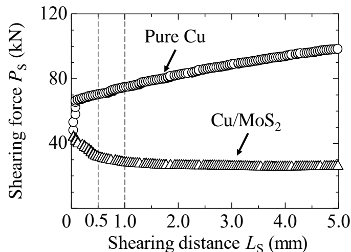
Fig. 3-21 Evolution of the shearing force as a function of the shearing distance.
