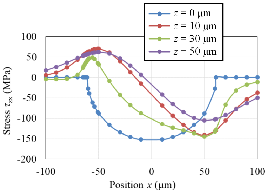
Fig. 4-15 Stress \tau_{zx} applied to pure Cu sample along x -axis ( P = 4.0 \text{ N} , \mu = 0.30 ) calculated by using Hamilton's model.
