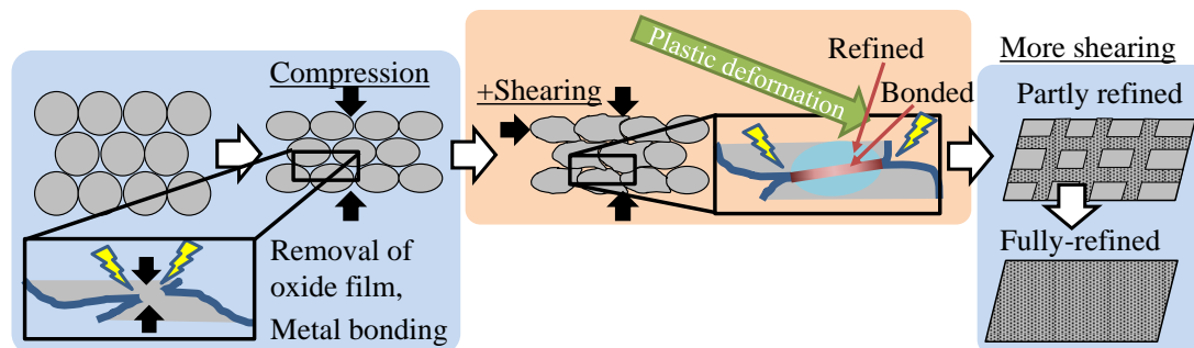
Fig. 5-1 Simplified Horita's model.
