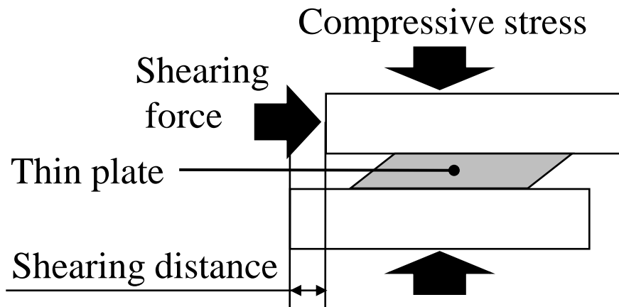
Fig. 3-2 Simplified schematic illustration of COSME-RT process.
