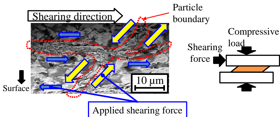
Fig. 5-7 Direction of applied shearing force to pure Cu powder particles in COSME-RT process of pure Cu sample.
