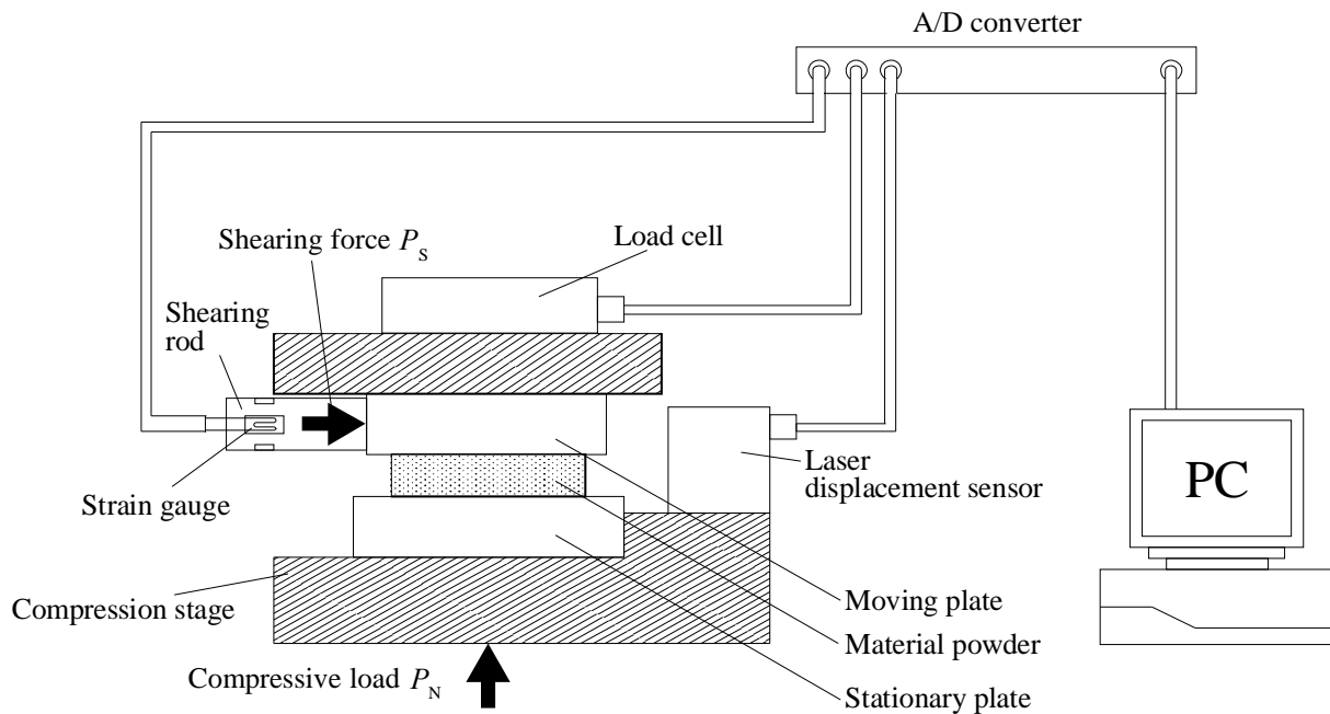
Fig. 2-5 Schematic illustration of compression shearing apparatus (DRD-NNK-002).
