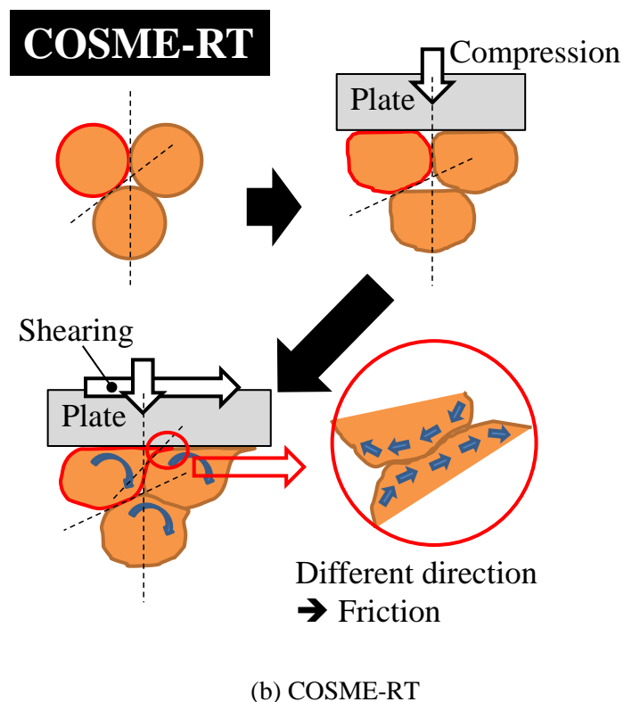
Fig. 5-9 Schematic illustration of bonding process of powder particles by (a) unidirectional friction experiment and (b) COSME-RT.
