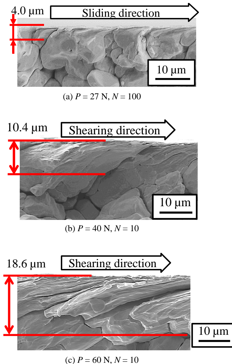
Fig. 4-8 SEM images of pure Cu sample fracture surfaces after friction experiments with different normal loads.
