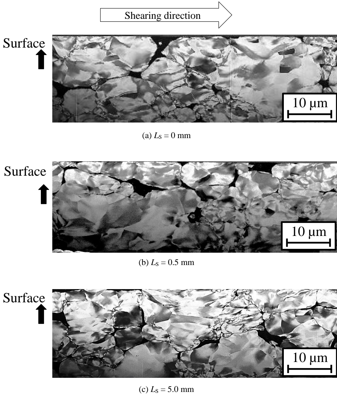
Fig. 3-19 SIM image of cross-section of Cu/MoS 2 samples (Top surface).
