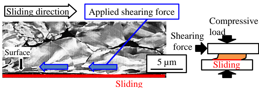
Fig. 5-6 Direction of applied shearing force to pure Cu powder particles in COSME-RT process of Cu/MoS 2 sample.
