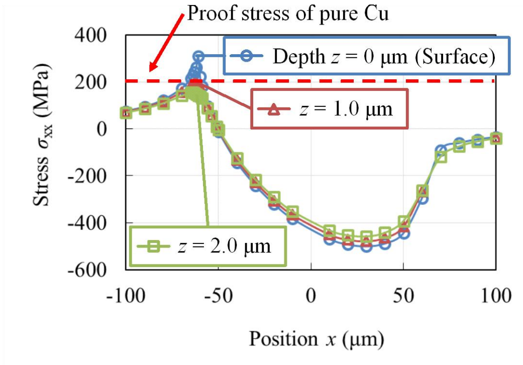
Fig. 4-14 Stress \sigma_{xx} applied to pure Cu sample along x -axis ( P = 4.0 \text{ N} , \mu = 0.30 ) calculated by using Hamilton's model.
