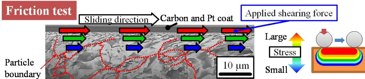
Fig. 5-5 Direction of applied shearing force to pure Cu powder particles in friction experiment.
