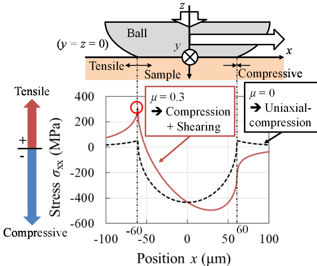
Fig. 4-13 Stress \sigma_{xx} along x -axis of circular contact for P = 4.0 \text{ N} , \mu = 0, 0.30 .
