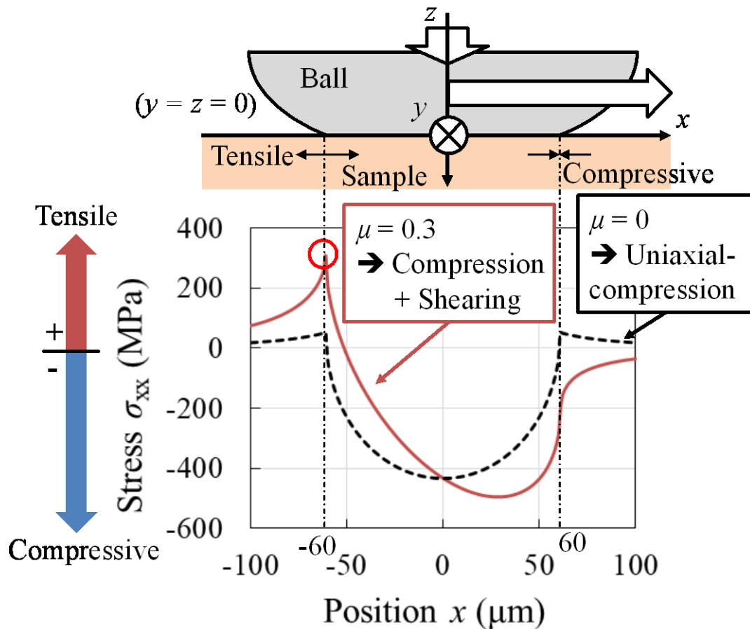
Fig. 4-13 Stress \sigma_{xx} along x -axis of circular contact for P = 4.0 N, \mu = 0, 0.30 .
