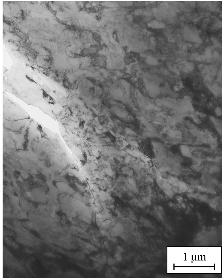
Fig. 3-14 TEM image of cross-section of r = 0 vol.% sample.
