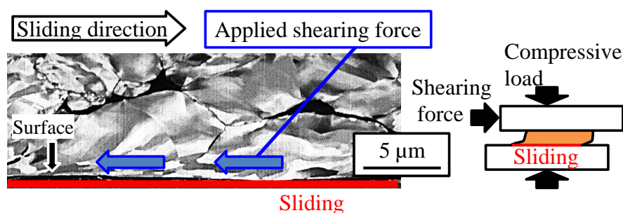
Fig. 5-6 Direction of applied shearing force to pure Cu powder particles in COSME-RT process of Cu/MoS 2 sample.
