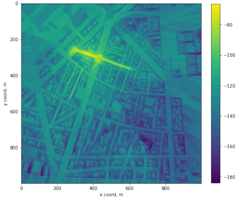
Figure 2.1: Example of signal strength distribution (in dBm) generated through Ray-Tracing in the Paris dataset, with respect to one particular base station roughly located in (300\text{m}, 300\text{m}) .
