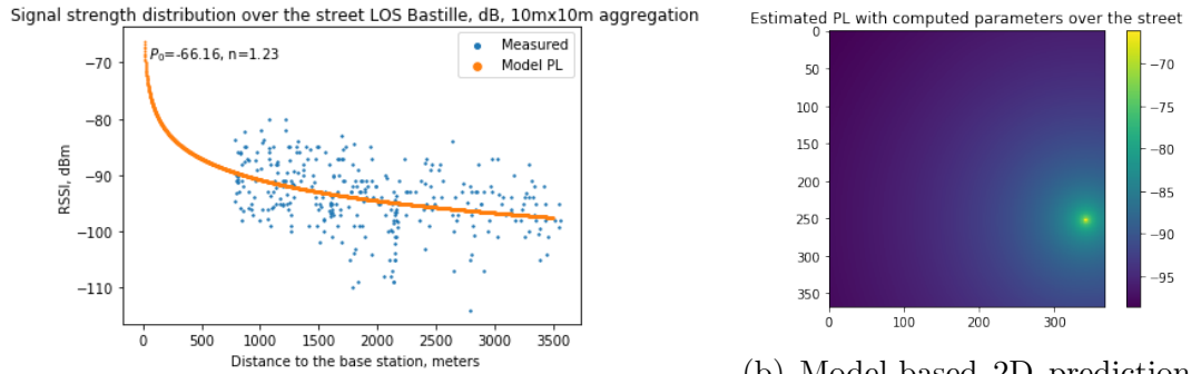
(a) RSS measurements distribution and model-based 1D average prediction in LoS, as a function of transmission range
