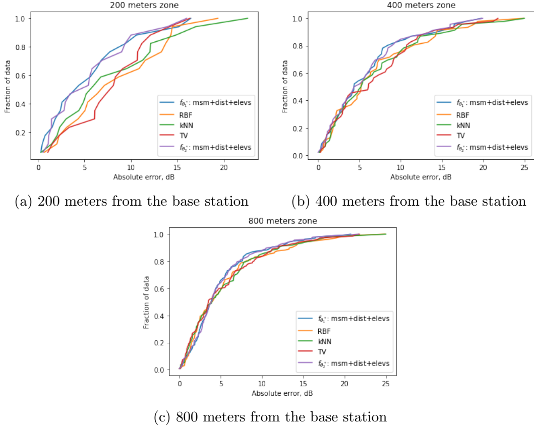
Figure A.9: ECDF plots of errors for the key distances over test Antwerp dataset. Comparison between baselines and NAS model trained over Antwerp dataset, BS'_g
