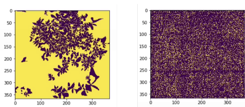
Figure A.3: Gradients behaviour over test base station. Binary mask of the points, where sum over x and y gradients is below some small value (for each axis less than 0.001; in yellow is small). Left : RBF interpolation, Right : GAN interpolation
