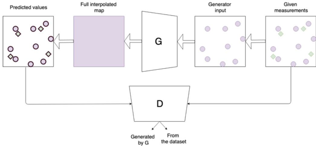
Figure A.1: Schema of learning procedure in GAN (specifically, measurements division). Training points from the masks M_l are given as an input to Generator (G) while in the Discriminator (D) we have both training and validation points from masks M_l and M_v
