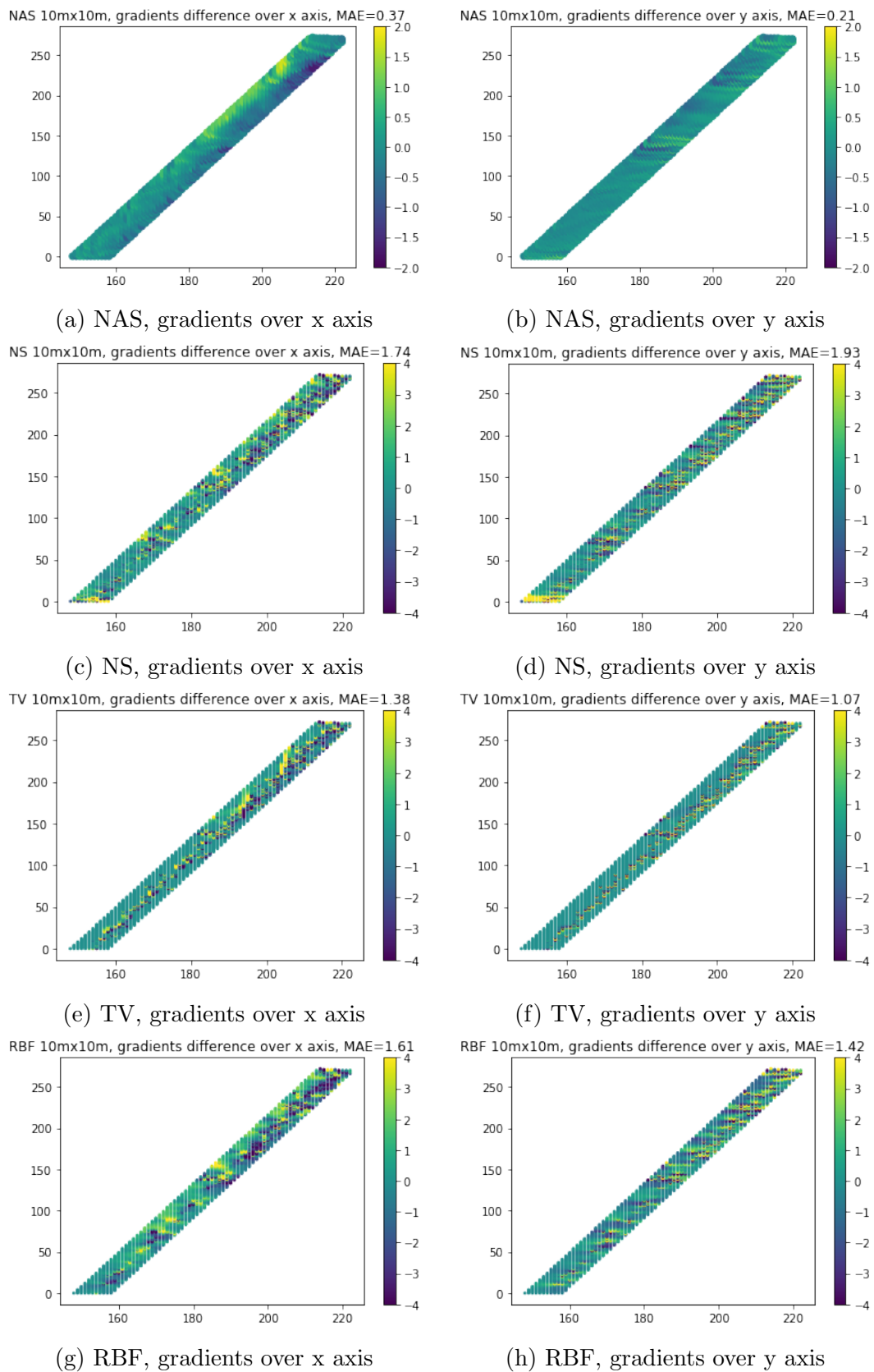
Figure 4.7: Difference between different methods gradients and signal distribution model gradients over LOS street
