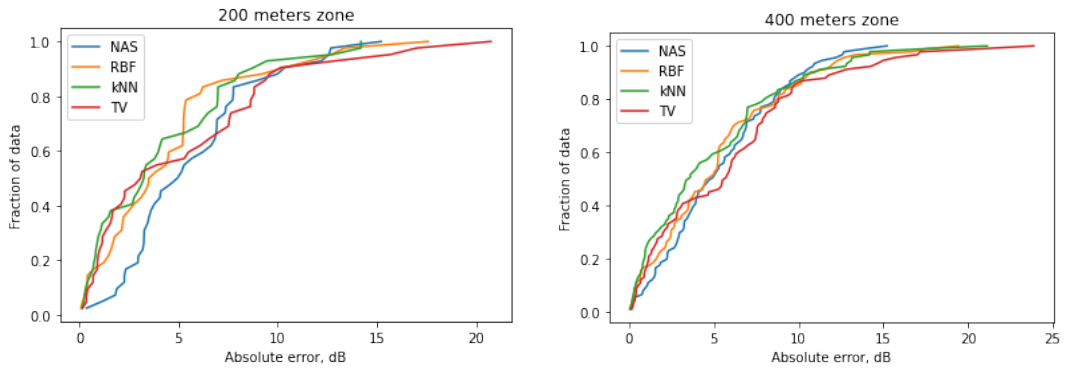
(a) 200 meters from the base station (b) 400 meters from the base station
