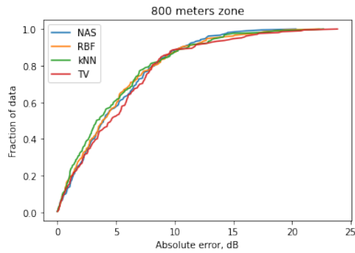
(c) 800 meters from the base station
