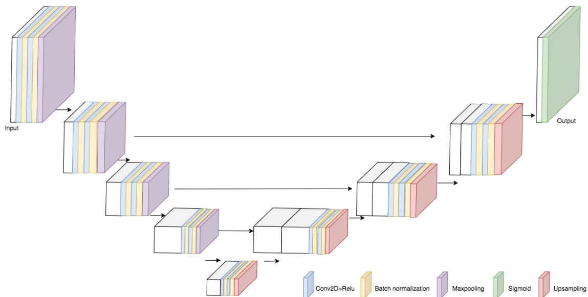
Figure 3.2: UNet-based architecture
