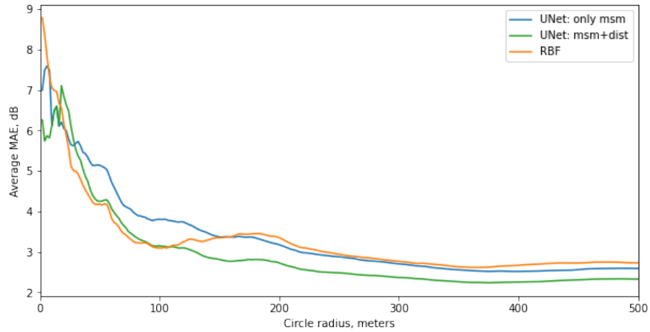
Figure 5.5: MAE for the distance from the base station for the RBF and fixed UNet outputs over Paris dataset with validation set compliment to the train one, measurements and distances or only measurements input
