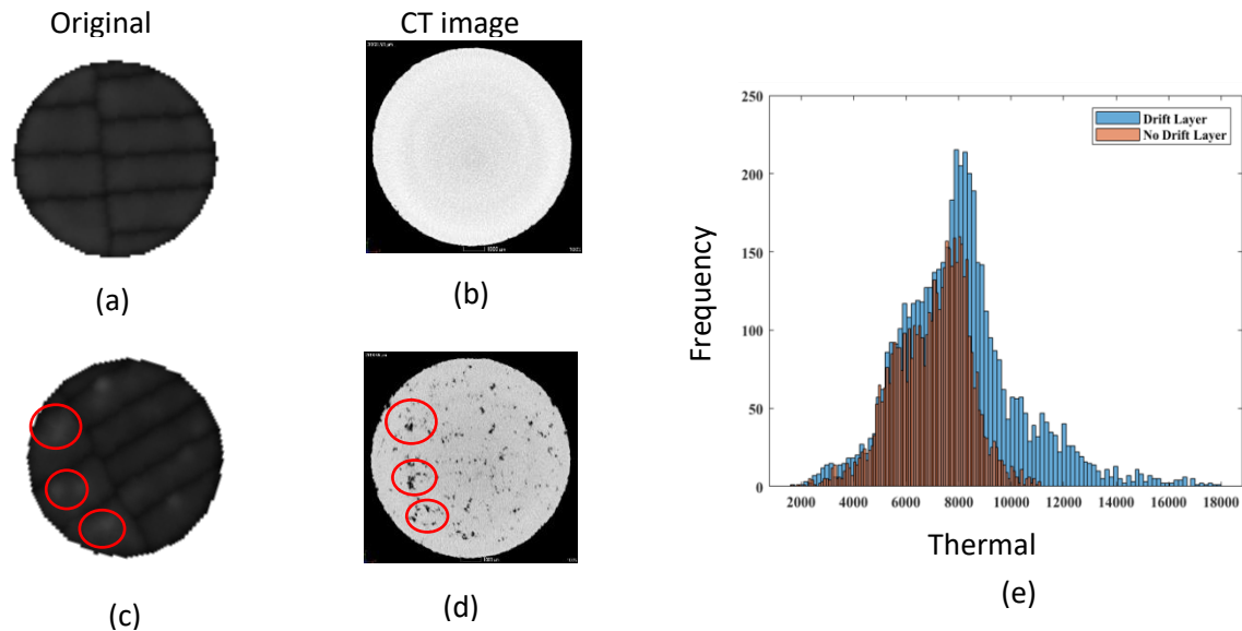
Figure 52: Example picture of (a) OT image without hotspots, (b) CT image of corresponding layer (a) without hotspots, (c) OT image with hotspots, (d) CT image of corresponding layer (c) with hotspots, and (e) histogram comparison between (a) and (c).
