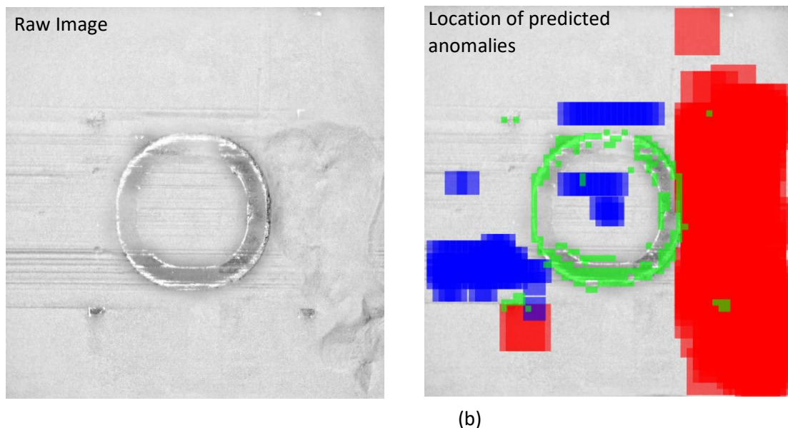
Figure 96: (a) The percentage of pre-exposure anomalies predicted by the CNN model along the build height, (b) An pre-exposure image example showing the exact location of predicted anomalies (Red: “Uneven Powder Spreading”, Green: “Part-Hopping”, and Blue: “Recoater streaking.”)
