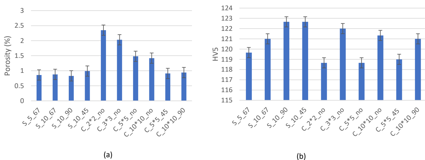
Figure 26: Effect of scanning strategies on (a) porosity (b) vicker's hardness.
