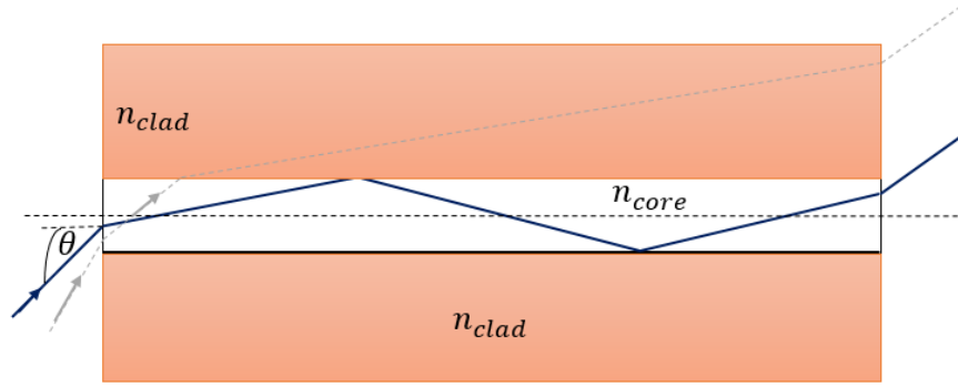
Figure 31: Total internal reflection into the fiber core
