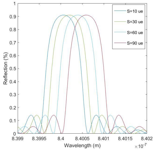
Figure 46: Bragg wavelength spectrum shift induced by axial strain in FBG
