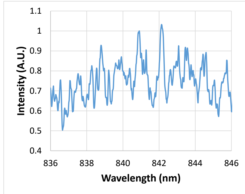
Figure 51: Zoom of the spectrum on the zone of interest
