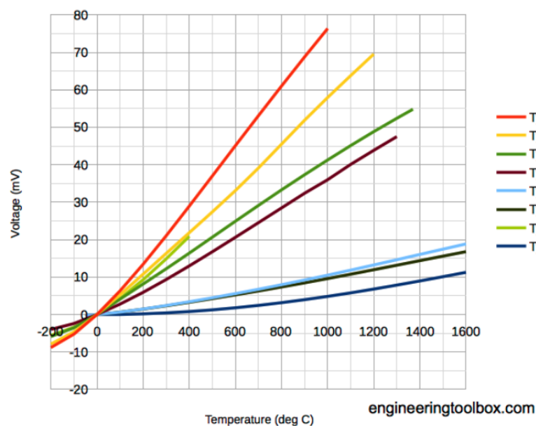
Figure 12: Voltage difference versus temperature characteristic curve of a thermocouple
