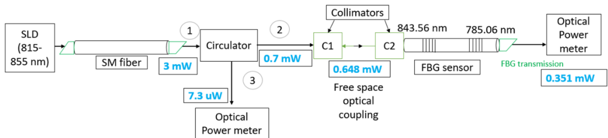
Figure 58: SLD coupling with circulator with the collimator lenses system
