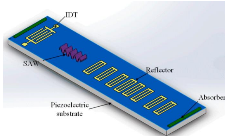
Figure 5: Schematic of a typical SAW device
