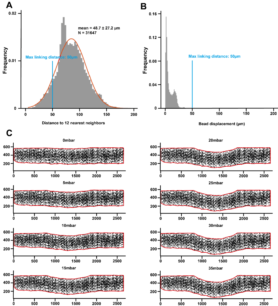
Figure 31: Preparing data for strain analysis.
