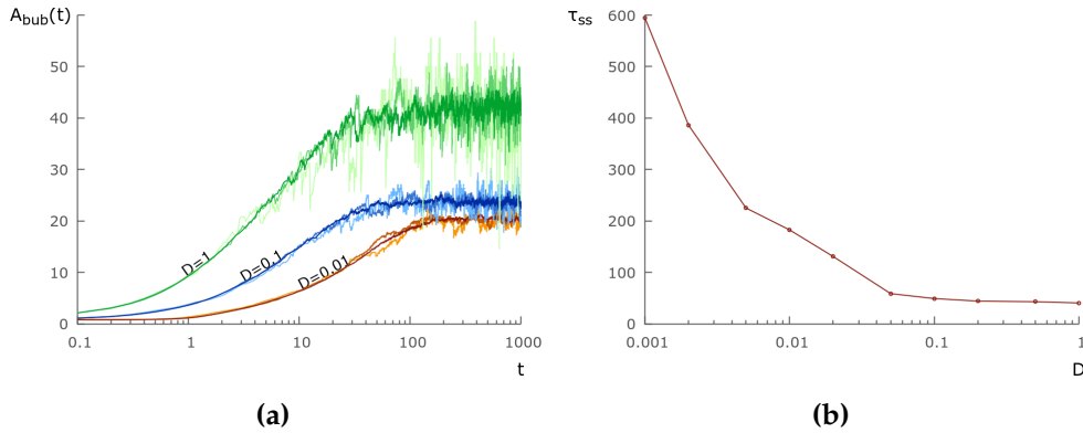
Figure 4.4: Behavior of the convergence time \tau_{ss} in the bubbly liquid ( v_g = 0.4 ) when varying the diffusivity D . (a) Time series of the average bubble size. For each diffusivity constant ( D = 0.01, 0.1, 1 ), we show three time series at different system sizes ( L = 50, 100, 200 , from light to dark color). As we can see, the convergence time does not depend on the system size while it depends on D . (b) From time series analogous to the one in (a) we extracted the convergence time \tau_{ss} as we described in Section 2.3.2 for AMB+. Notice how the convergence time decreases when increasing D .
