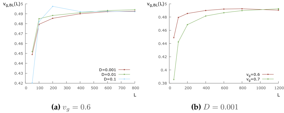
Figure 4.8: Steady-state vapor fraction in the bubbly liquid as a function of the linear system size L .
