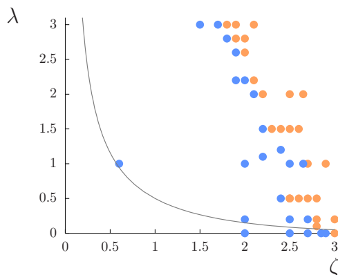
Figure A.1: Region of the \zeta \times \lambda phase space in which the code is stable with accuracy dt = 2 \times 10^{-2} and dx = 1 (blue dots). Tests are done for system dimensions L = 256 \times 128 , at high noise ( D = 0.3 ). The solid line represents the transition between reverse and direct Ostwald ripening process.
