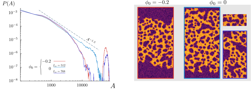
Figure 2.18: Left: intermediate power law of the bubble size distribution P(A) \sim A^{-1.5} for D = 0.25, \phi_0 = 0, L_x = 512 = 2L_y . Notice how we pass from a bubbly liquid state for small sizes (less than 512 \times 256 ) to a bubbly phase separated state by increasing system size. In red we represent for comparison the converged P(A) of the bubbly liquid state at \phi_0 = -0.2 .
