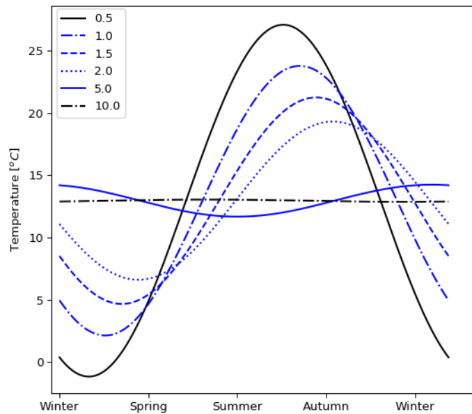
Figure 2.11: Ground temperature representation for various depths.
