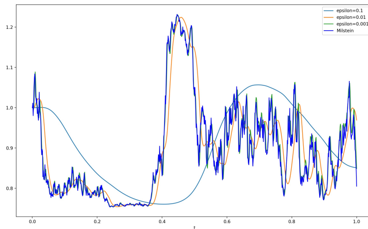
Figure 3.2 – AP scheme for different values of \varepsilon , with \sigma(x) = \cos(2\pi x) , \Delta t = 1.10^{-3} , and comparison with Milstein scheme.
