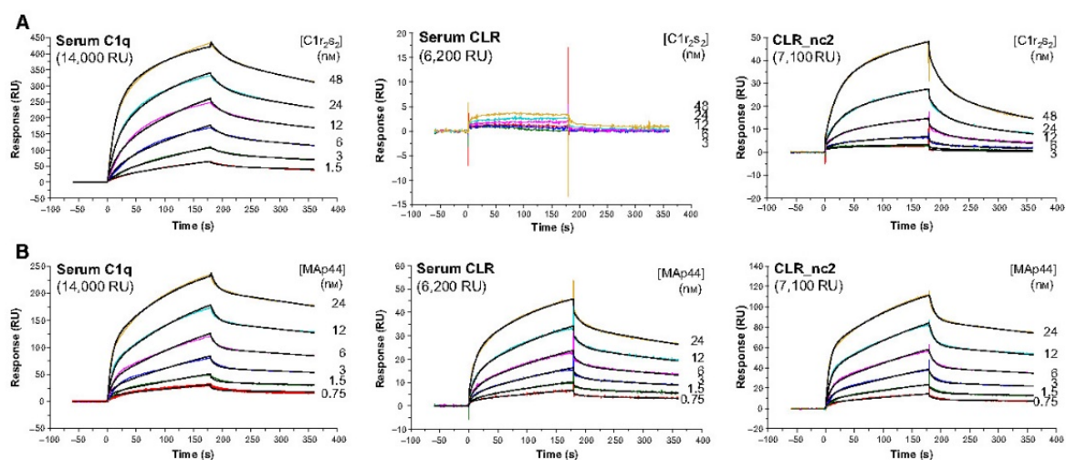
Fig. 6. Kinetic analysis of the interaction of C1r2s2 and MAP44 with immobilized serum C1q, serum CLR and CLR_nc2. C1r2s2 (A) and MAP44 (B) were injected at the indicated concentrations over immobilized serum C1q (14 000 RU) (left), serum CLR (6200 RU) (middle), and CLR_nc2 (7100 RU) (right) at a flow rate of 30 \mu\text{L}\cdot\text{min}^{-1} in 50 mM Tris/HCl, 150 mM NaCl, 2 mM \text{CaCl}_2 , 0.05% surfactant P20 (pH 7.5). Fits obtained by a global fitting of the data to a two-state reaction model are shown in black. The results shown are representative of four (C1r2s2) or two (MAP44) experiments (Table 1).
