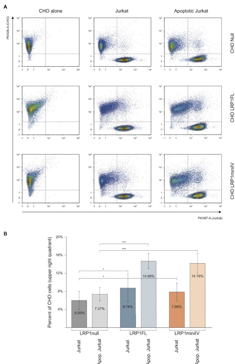
FIGURE 9 | Flow cytometry analysis of the interaction of Jurkat apoptotic cells with LRP1 full-length and mini IV CHO cells. (A) Dot plots of the analysis of PKH26 fluorescent CHO cells (red, Y4-A channel) decorated by PKH67 fluorescent Jurkat cells (green, B1-A channel). Decoration efficiency is calculated in the upper quadrant of the region drawn, as the percentage of PKH26 positive events (B) Histograms obtained from 13 independent experiments. Student T test relevance is shown above the histograms. *** Student bilateral unpaired <1 \times 10^{-2} , * Student bilateral unpaired <2 \times 10^{-1} .
