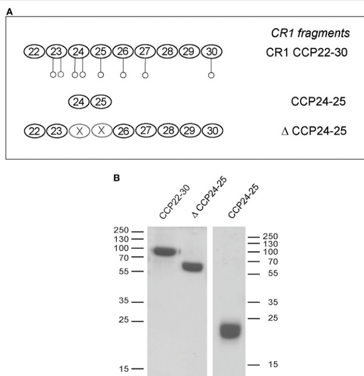
FIGURE 3 | Complement receptor type 1 (CR1) variants produced to study the CCP24-25 module pair interaction properties. (A) Schematic view of CCP24-25 variants produced in eukaryotic cells. Potential N-glycosylations are represented by open circles \circ . (B) SDS-PAGE analysis of 4 \mu g of the CR1 variants under reducing conditions. The positions of the molecular weight markers (expressed in kilodaltons) are indicated. A full scan of the original gel is provided in Figure S1 in Supplementary Material.
