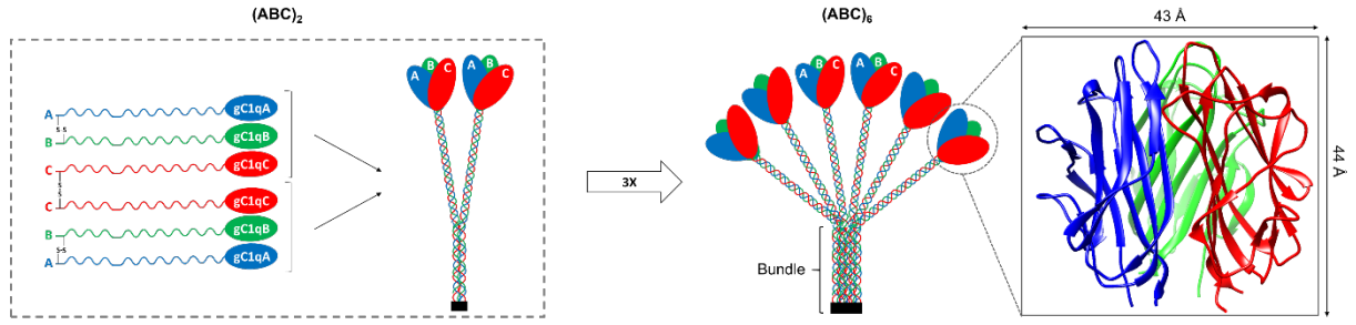
Figure 3: Schematic representation of C1q assembly. The C1q molecule is assembled from 18 polypeptide chains of three different types (A, B and C) each containing an N-terminal collagen-like sequence and a C-terminal globular domain (gC1q). Six C1q chains assemble into the (ABC) 2 sub-unit that then trimerizes into the full-length (ABC) 6 C1q exhibiting its characteristic bouquet-like shape with six C-terminal globular regions (GR) linked together through six collagen-stems (CLR) assembled into an N-terminal bundle. The right panel shows the crystal structure of C1q GR (PDB code: 1PK6). (Taken from Fouët et al. 2020a; Article 1).
