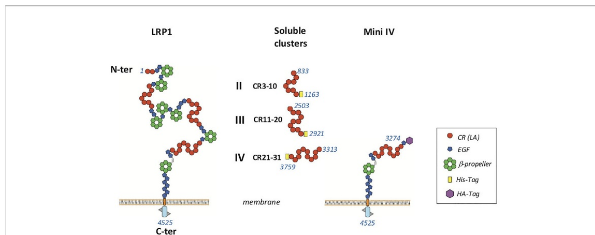
FIGURE 1 | Schematic representation of LRP1 fragments used in this study. LRP1 clusters II, III and IV were produced in 293-F mammalian cells with a His-Tag at the C-terminal extremity. Membrane full-length LRP1 and minireceptor IV (mini IV) were used for cellular interaction studies. CR, complement repeat; LA, LDL receptor class A; HA, hemagglutinin; EGF, epidermal growth factor. Amino acid numbering of mature LRP1 is indicated in blue.
