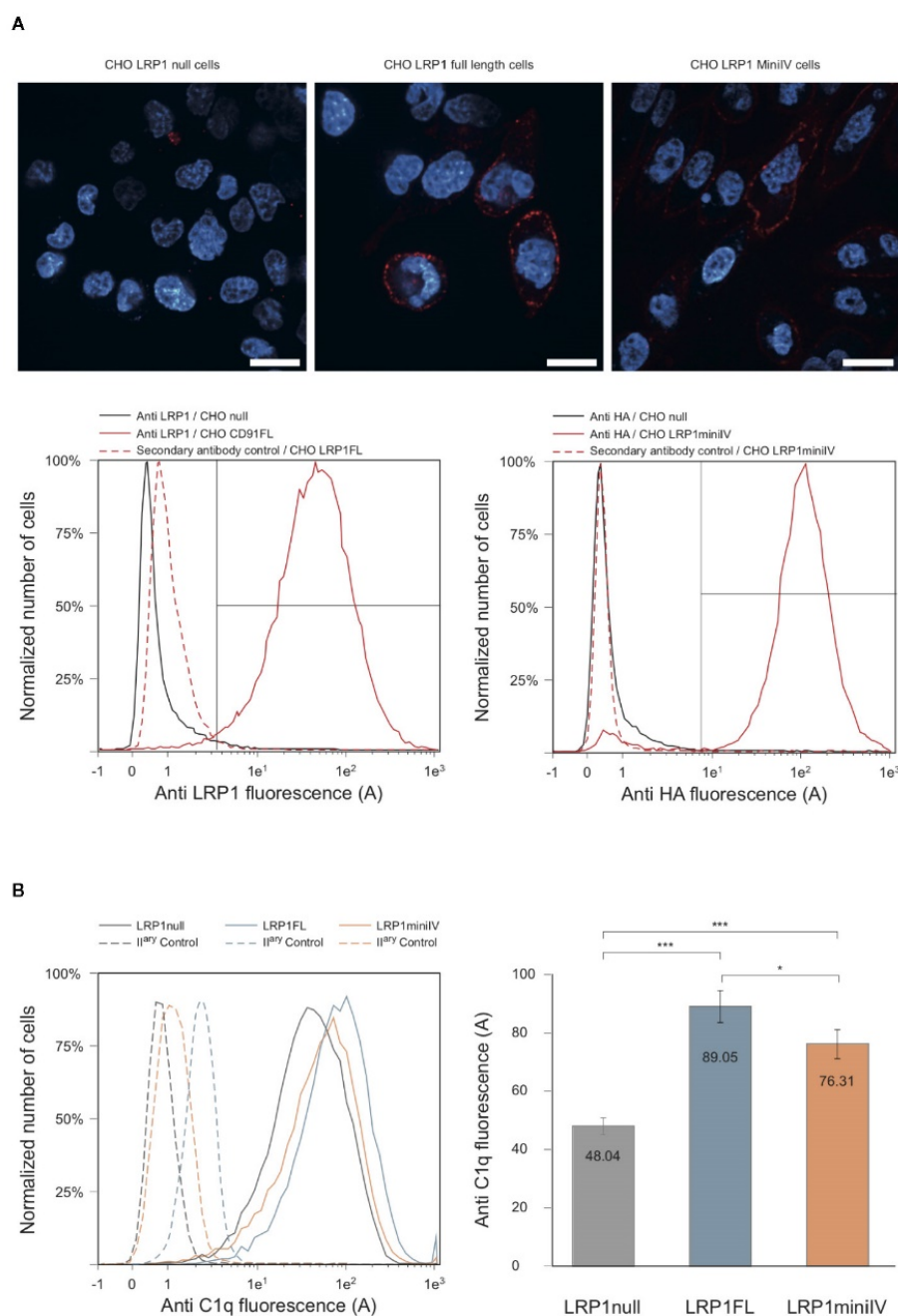
FIGURE 8 | C1q interacts with full-length LRP1 and mini IV at the surface of transfected CHO cells. (A) Antibody labeling of LRP1-null CHO cells and CHO cells transfected with full-length LRP1 or mini IV. Top panels, confocal sectioning of LRP1-null, full-length LRP1 and mini IV (red) DAPI counterstained (blue) adherent CHO cells (bars = 20 \mu m). Bottom panels, histogram overlays of the corresponding cell populations analyzed by flow cytometry. Left, control LRP1-null cells (black) and LRP1 full-length transfected CHO cells (red) labeled with anti LRP1 antibody. Right panel, control LRP1-null CHO cells (black) and mini IV transfected CHO cells (red) labeled with anti HA antibody. Red dotted histograms correspond to secondary antibodies controls. The region for positive cells is shown (brackets) and represents more than 95% of the total cell population. (B) Flow cytometric histograms of a typical C1q decoration experiment. Plain lines correspond to C1q binding to LRP1-null cells (grey), full-length LRP1 (blue) and mini IV (red) CHO cells. Dashed lines are the corresponding controls with only secondary antibody only. Right pane, mean C1q fluorescence intensities (corrected from the controls) of six independent experiments. *** Student bilateral unpaired <1 \times 10^{-4} . * Student bilateral unpaired >4 \times 10^{-2} .
