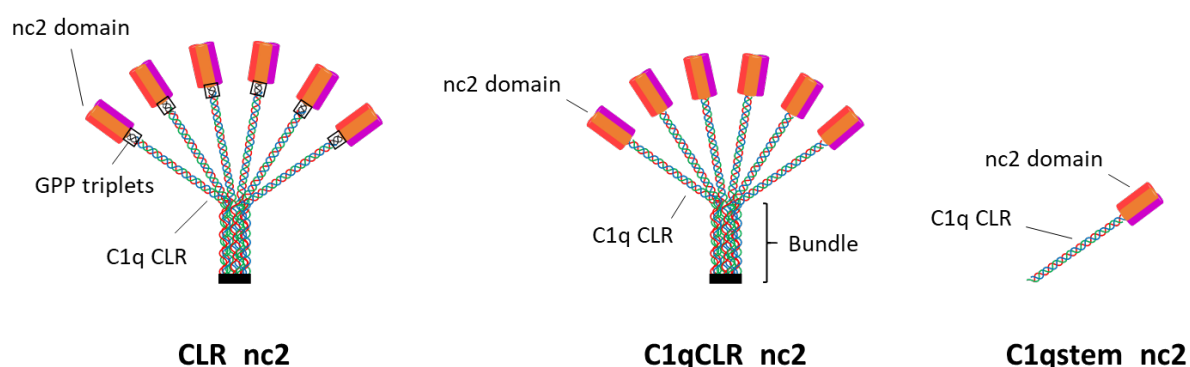
Figure 21: Schematic representation of the CLR_nc2 (left), C1qCLR_nc2 (middle) and C1qstem_nc2 (right). The nc2 domains are represented as red, orange and purple cylinders, the additional GPP triplets inserted into the CLR_nc2 are colored in black and the C1q collagen chains are shown in red, blue and green.
