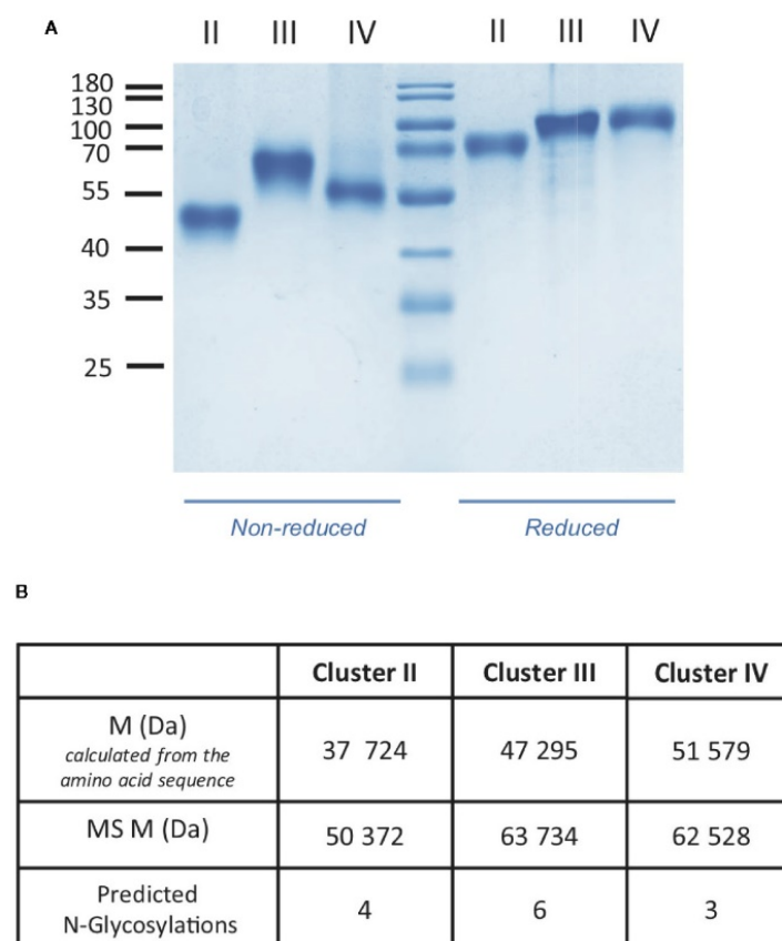
FIGURE 2 | Characterization of LRP1 clusters. (A) SDS-PAGE analysis of LRP1 clusters. Clusters II, III and IV in non-reducing (left) and reducing conditions (right), molecular weight markers are indicated in kDa. (B) , MALDI mass spectrometry analysis of LRP1 clusters. M, molecular weight; MS, Mass spectrometry.
