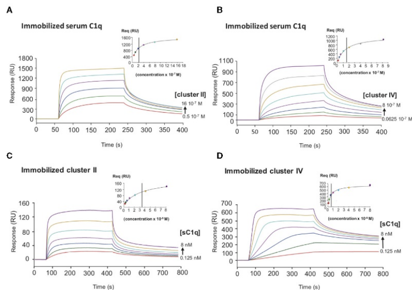
FIGURE 5 | Comparative kinetic analysis of the interaction of serum C1q with LRP1 clusters II and IV. SPR analysis of LRP1 clusters II and IV interactions with serum C1q in two configurations. Top panels, clusters II and IV were injected over immobilized serum C1q (14,000 RU). (A, B) respectively. Bottom panels, serum C1q was injected over immobilized clusters II (1,230 RU) and IV (1,270 RU), (C, D) respectively. All injections were performed in 50 mM Tris, 150 mM NaCl, 2 mM CaCl 2 , 0.05% P20, pH 7.4. The concentration of soluble ligands is indicated on each curve. The Req versus concentration plots of steady state fittings are shown on the top right of the SPR curves. K_D values (means \pm SD) for each kinetics are summarized in Table 2 .
