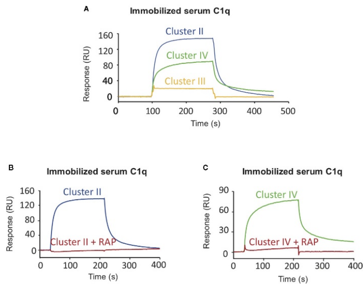
FIGURE 4 | LRP1 clusters II and IV interact with C1q. SPR analysis of LRP1 clusters II (blue curves), III (yellow curves) and IV (green curves) interactions over immobilized C1q, in the presence or absence of RAP. Clusters II, III and IV (500 nM in 50 mM TEA, 150 mM NaCl, 2 mM CaCl 2 , 0.005% P20, pH 7.4) were injected over immobilized serum C1q (17,500 RU) with or without RAP (500 nM). (A) comparison of the interaction curves in the absence of RAP for clusters II, III and IV. (B, C) Comparison of the binding of Cluster II (B) and Cluster IV (C) in the presence or in the absence of RAP.
