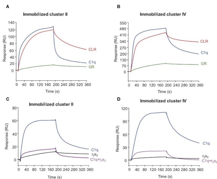
FIGURE 6 | The interaction site of LRP1 clusters II and IV on C1q is located on the collagen stalks at or close to the site interacting with C1r2s2 tetramer. C1q (10 nM, blue curves), CLR (10 nM, red curves) and GR (60 nM, green curves) were injected over immobilized LRP1 cluster II (1,230 RU, A panel) or LRP1 cluster IV (1,270 RU, B panel), in 50 mM Tris, 150 mM NaCl, 2 mM CaCl 2 , 0.05% P20, pH 7.4. C1q (1 nM) was injected on the same amount of clusters II and IV (bottom C , D ) with (pink curves) or without (blue curves) C1r2s2 (1 nM). r2s2 was also injected alone (1 nM) as a reference (black curves).
