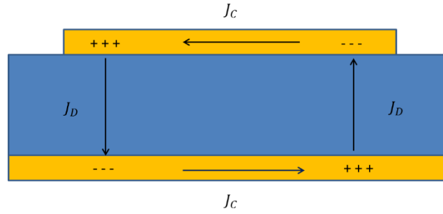
Figure 2.1.2 Illustration of a magnetic moment resulting from the excitation of electrical dipoles in antiparallel configurations in the top and bottom metal layers tightly coupled via an ultra-thin dielectric substrate.
