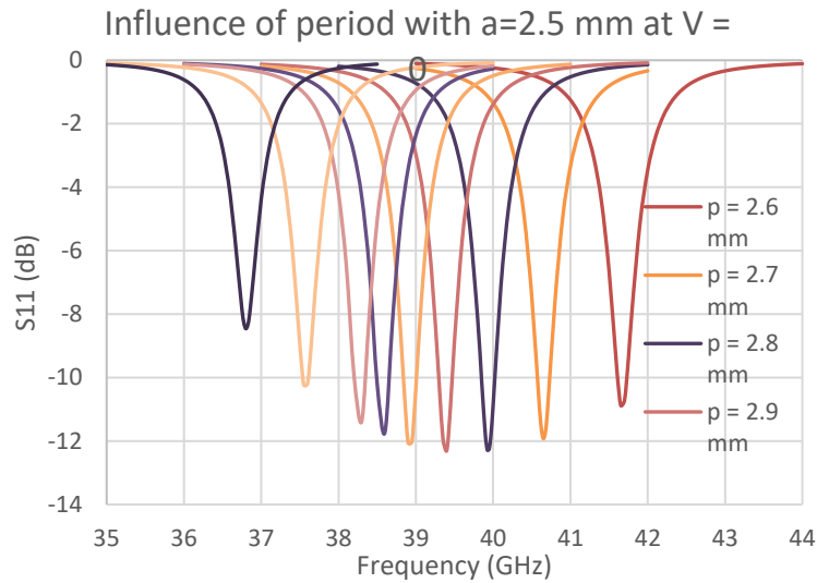
Figure 3.1.15 Influence of the period on the frequency response of the model when V = 0 . LC 5CB ( t_{LC}=10\ \mu\text{m} , \epsilon_{rL}=2.64 , \text{tg}\delta=0.014 ), w_{\text{int}}=150\ \mu\text{m} , t_{\text{glass}}=1.1\ \text{mm} , \epsilon_{\text{glass}}=5.7 and a=2.5\ \text{mm}
