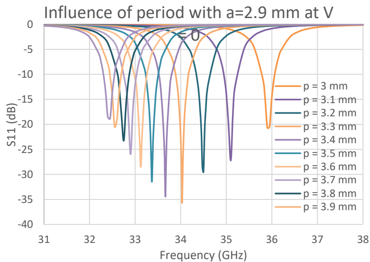
Figure 3.1.16 Influence of the period on the frequency response of the model when V = 0 . LC 5CB ( t_{LC}=10\ \mu\text{m} , \epsilon_{rL}=2.64 , \text{tg}\delta=0.014 ), w_{\text{int}}=150\ \mu\text{m} , t_{\text{glass}}=1.1\ \text{mm} , \epsilon_{\text{glass}}=5.7 and a=2.9\ \text{mm}
