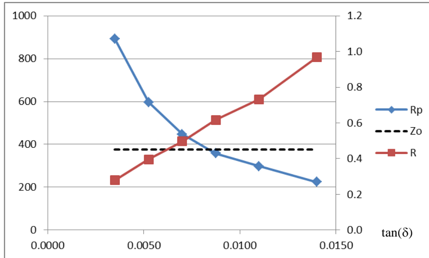
Figure 3.2.18 Influence of the LC dielectric losses \text{tg}\delta on the resistance R , R_p with p=5 mm, the dielectric permittivity \epsilon=3(1-j0.014) and the dielectric thickness t=50 \mu\text{m}
