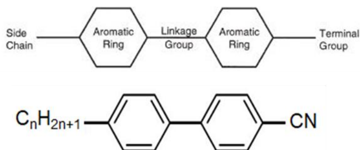
Figure 1.1.4 Typical structure of rod-like LC and example of p - n alkyl- p' -cyanobiphenyls [9]
