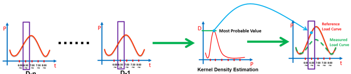
Figure IV.3 Formulation of reference load curve using Kernel Density Estimation
