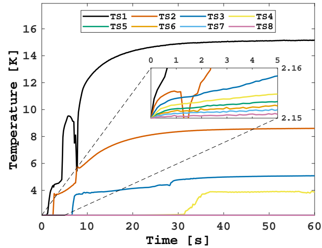
(a) q = 279.5 \text{ kW/m}^2
