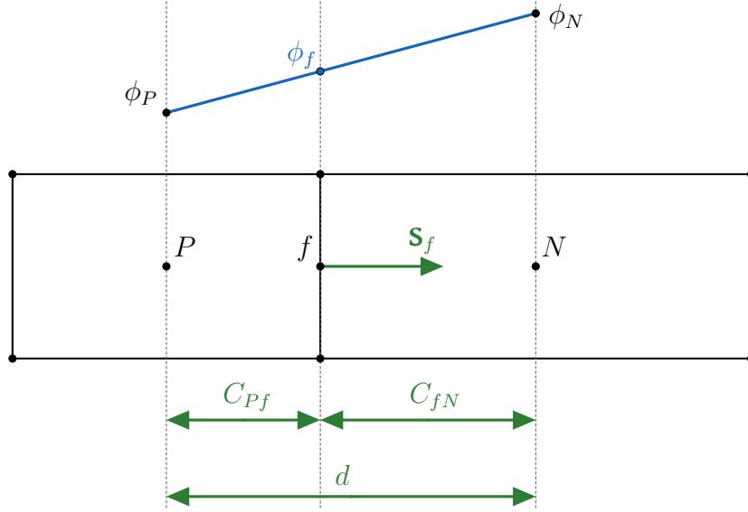
Figure 3.15: Schematic representation of two adjacent cells in a non-uniform orthogonal grid.
