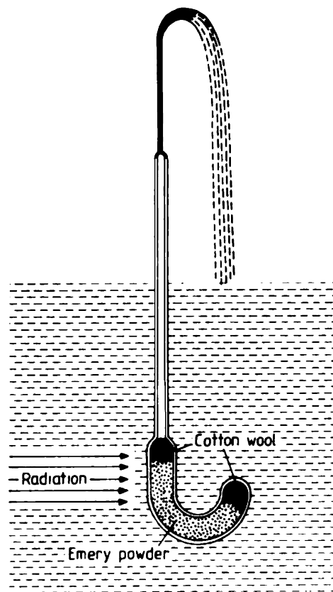
Figure 2.3: Schematic representation of the experimental apparatus used by Allen and Jones [4] to show the fountain effect [167].
