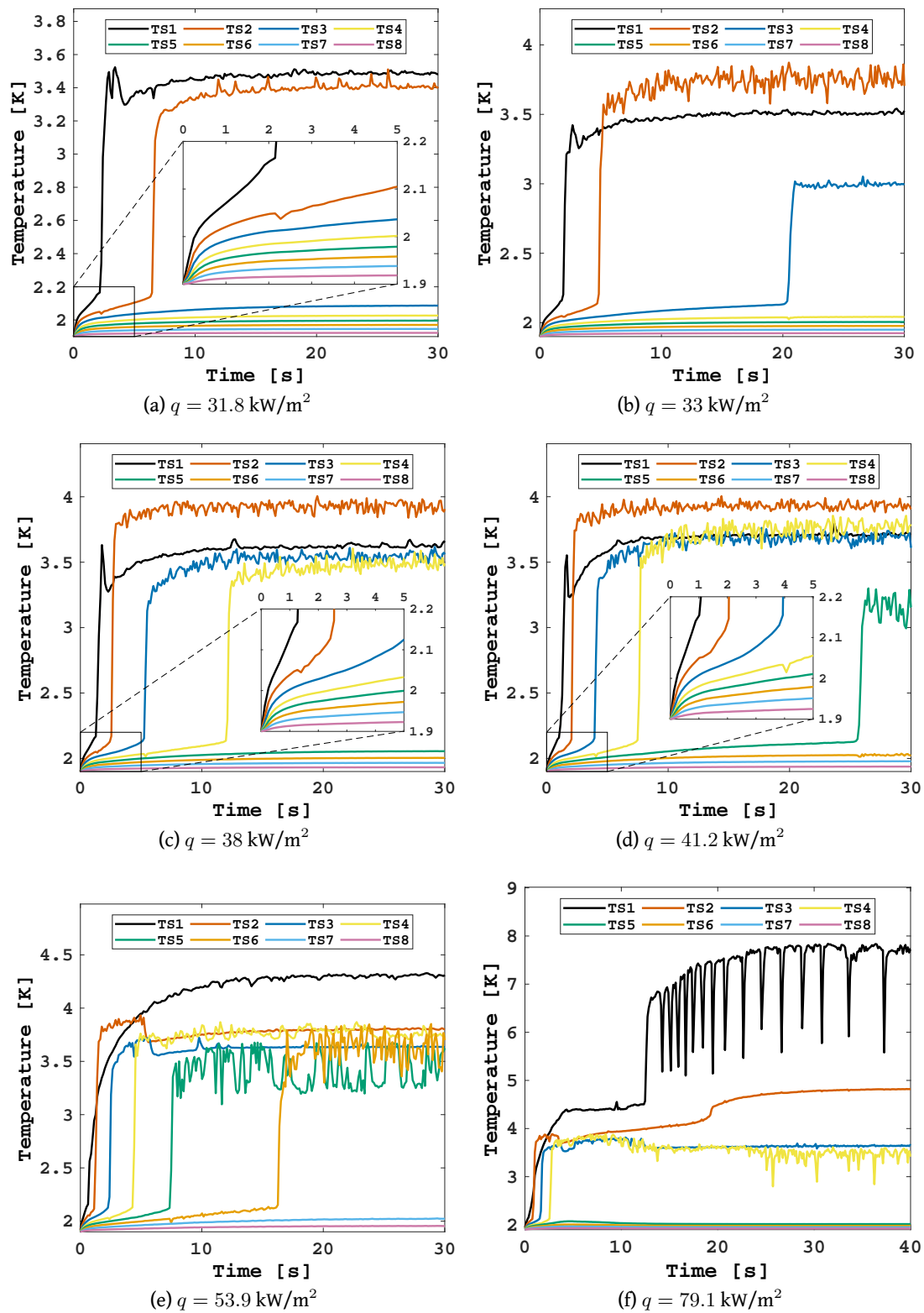
Figure A.5: Temperature evolution in the horizontal 0.2 mm thick channel at T_b = 1.9 \text{ K} and different heat fluxes q .
