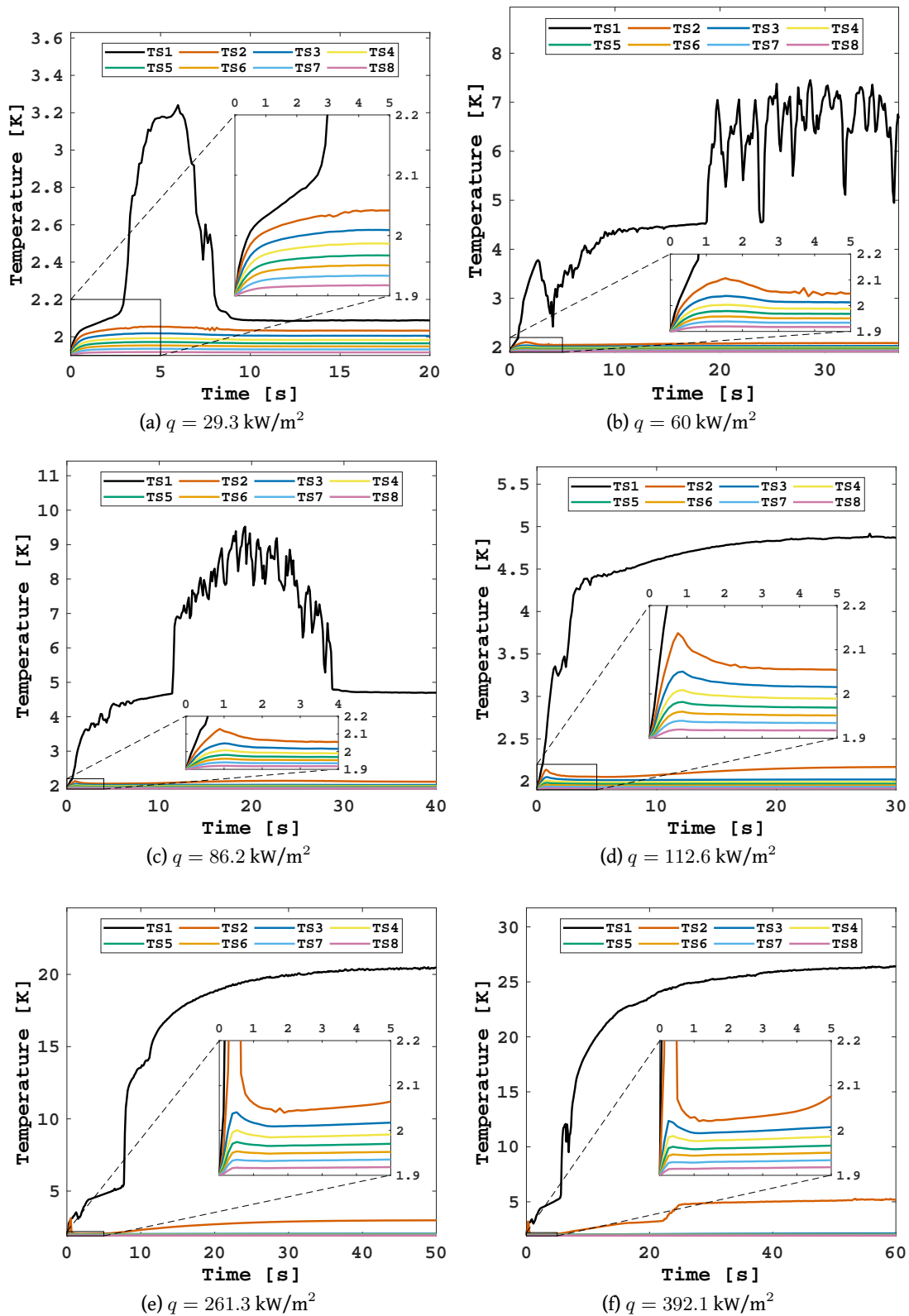
Figure 5.6: Temperature evolution in the horizontal 0.5 mm thick channel at T_b = 1.9 \text{ K} and different heat fluxes q .
