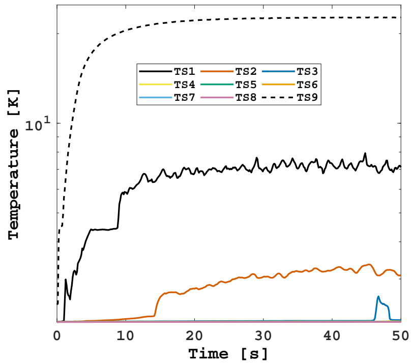
Figure A.14: Temperature evolution in the horizontal 0.5 mm thick channel at T_b = 2.15 K and the heater at 22.7 K.
