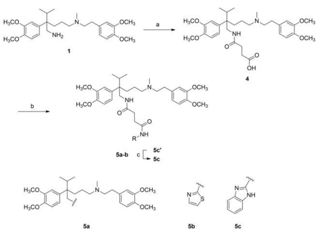
Scheme 3. Synthetic procedure for the synthesis of compound 4 bearing a succinamic acid linker and of amide-linked derivatives 5a–c . Reagents: a) succinic anhydride, CH 2 Cl 2 , r.t., overnight; b) amine, HOBT, EDC, Et 3 N, CH 2 Cl 2 , r.t., overnight; c) TFA, CH 2 Cl 2 , r.t., overnight.
