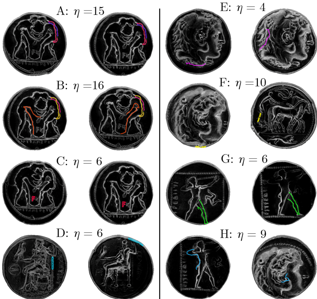
Figure 3.27: Some results of the retrieval for target coins. The extraction has been performed with the skeleton map. Corresponding scores are written above the matching pair. Coins in A, B, C and E are correctly paired although the pairing of E does not stem from a good contour match.
