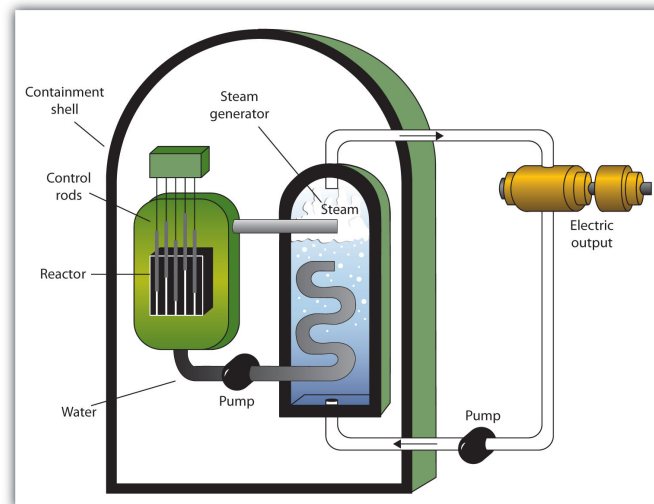
Figure 1.2: Schematic representation of nuclear power plant infrastructures [5].
