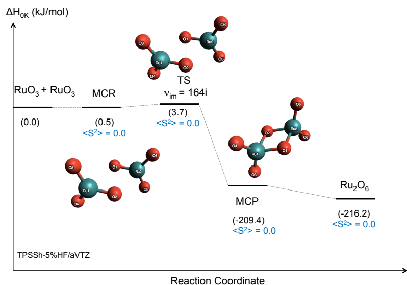
Figure 6.3: Reaction profile at 0 K calculated at the TPSSh-5%HF/AVTZ level of theory for reaction 2 \text{RuO}_3 \longrightarrow \text{Ru}_2\text{O}_6 with schematic representations of the intermediate species involved.
