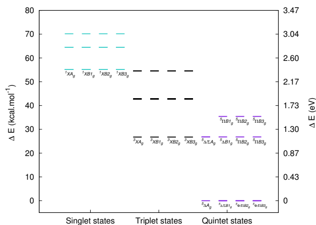
Figure B.1: Ru electronic spectra derived with MCSCF calculations. Fundamental energy is equal to -93.80139924 au for the 7 degenerated states ^5\Delta_{A_g} , ^5\Delta_{B_{1g}} , ^5\Sigma_{B_{1g}} , ^5\Phi_{B_{2g}} , ^5\Pi_{B_{2g}} , ^5\Phi_{B_{3g}} and ^5\Pi_{B_{3g}}
