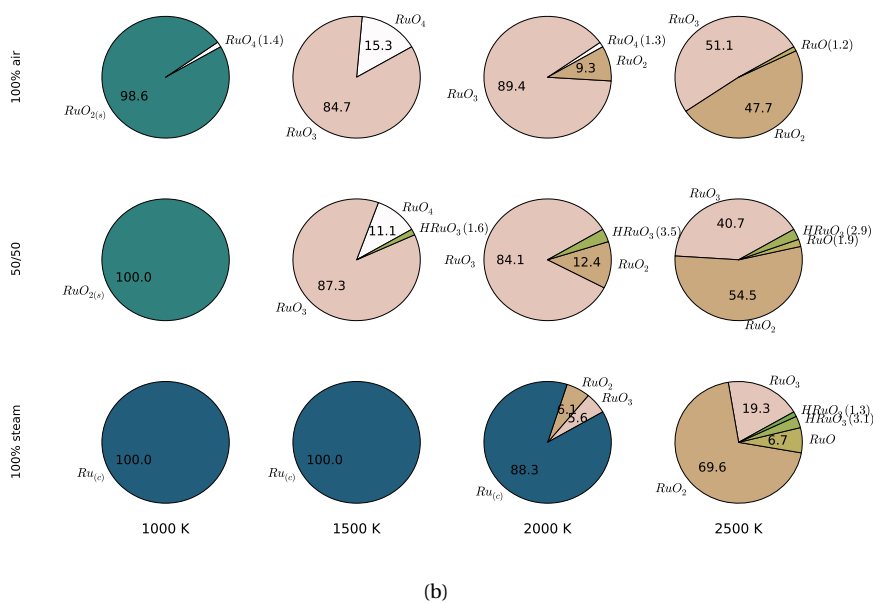
Figure 5.8: Ruthenium speciation (HRuO 3 and HRuO 2 correspond respectively to the RuO 2 (OH) and RuO(OH) gaseous species) for the release of 0.1 (a) and 0.01 (b) mol of ruthenium into a 0, 50 and 100 % steam-air mixtures, at a pressure of 2 bar in volume equal to 1 m 3 at different temperatures a .
