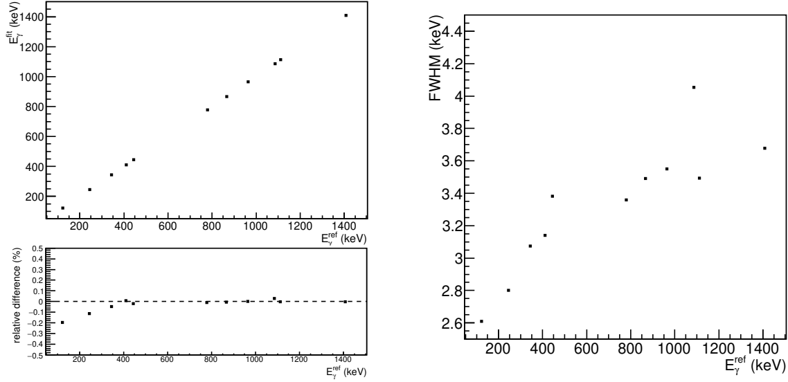
Figure 3.17: The energy resolution of AGATA from a ^{152}\text{Eu} source. Top left plot: the centroids from Gaussian fits ( E_{\gamma}^{\text{fit}} ) along the expected \gamma -ray peak energies ( E_{\gamma}^{\text{ref}} ) from [106]. Bottom left panel: the relative difference E_{\gamma}^{\text{ref}} - E_{\gamma}^{\text{fit}} derived, demonstrating the excellent calibration: at worst 0.2 % difference. The observed systematic differences for low \gamma -ray energies ( E_{\gamma} < 400 keV) were due to a remaining Compton background noise contribution which is usually important in the low energy region for HPGe crystals. Right panel: the evolution of the peak FWHM along the expected energy, with \text{FWHM} = 2.35 \times \sigma from Gaussian fits.
