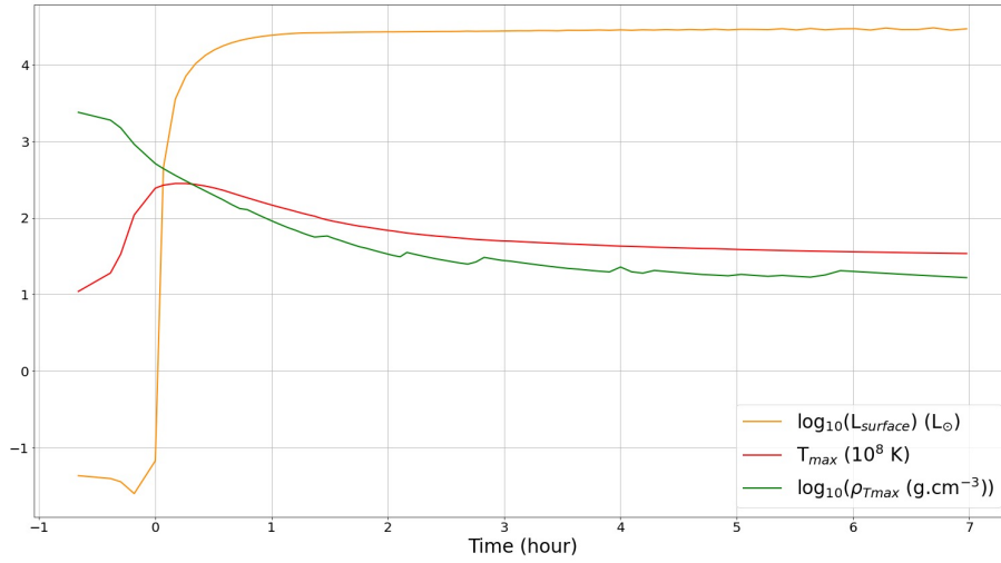
Figure 9.2: Set-up of the outburst during a ONe nova, simulated with MESA. Red curve: the maximum temperature T_{\max} plotted along the time, put at 0 for the peak temperature. Orange curve: the surface luminosity ( L_{\text{surface}} ). Green curve: the density at T_{\max} ( \rho_{T_{\max}} ). The outburst appears with a peak in T_{\max} , up to T_{\text{peak}}=0.24 GK, and a fast increase in L_{\text{surface}} , for less than 1 hour. This is followed by the constant bolometric luminosity stage ( L_{\text{surface}}=10^{4.4} L_{\odot} ). Units in the legend.
