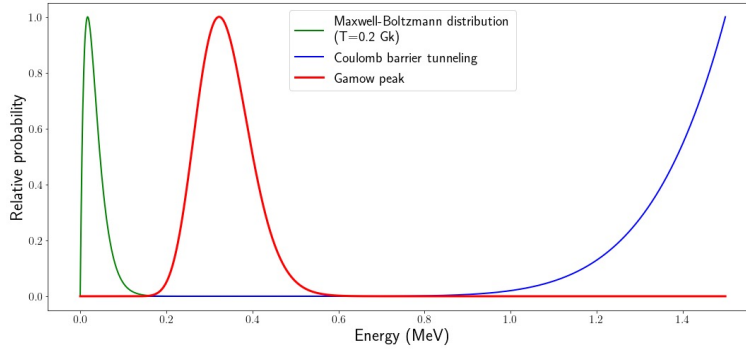
Figure 1.10: The Maxwell Boltzmann energy distribution calculated for T=0.2 GK (green curve) and the Coulomb barrier tunneling probability for the proton capture of ^{22}\text{Na} nucleus (blue curve) are shown as a function of the kinetic energy. The red curve is the product of the MB energy distribution and the cross section. This resulting Gamow peak represents the energy window where reactions are likely to occur.
