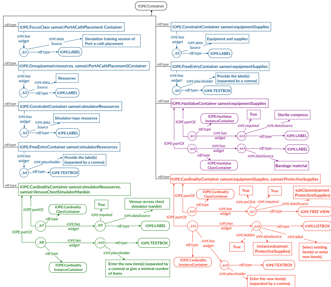
FIGURE 4.13: Illustration of IOPEWEB graph as the outcome of applying the mapping rules on the following example constraints: (\text{samsei:simulatorResources } \min 1 \text{ samsei:VenousChestSimulatorManikin}) , (\text{samsei:equipmentSupplies } \min 1 \text{ samsei:ProtectiveSupplies}) , and (\text{samsei:equipmentSupplies value samsei:sterile-compress}) .
