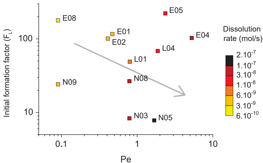
FIGURE 3.9 – Dissolution rate of each sample, depending on the initial formation factor F_L and the Péclet number Pe applied during the experiments. The color scale shows darker colors for higher dissolution rates R .
