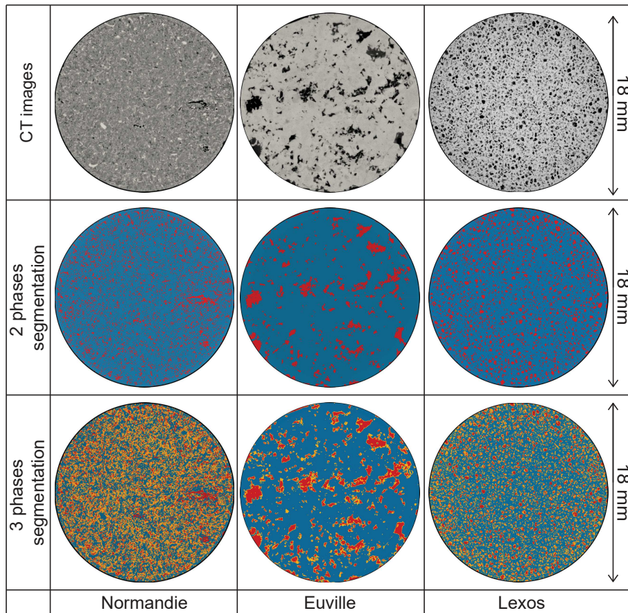
FIGURE 1.2 – 2D slices obtained from 3D XRMT images. Blue color represents the matrix phase, red the macro-phase and orange the micro-phase.
