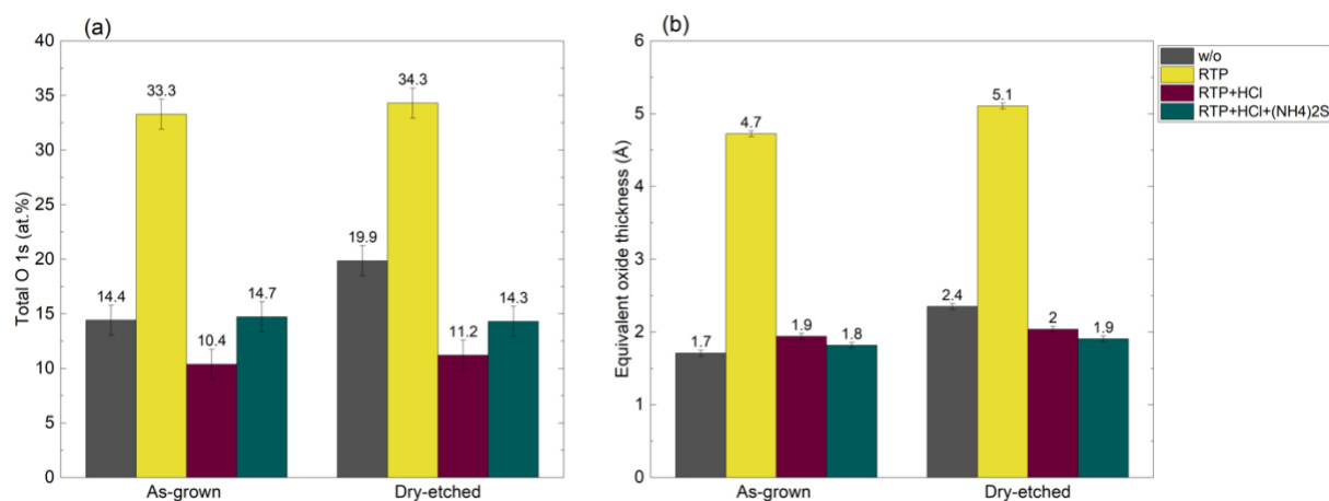
Figure 84. Impact of the RTP annealing followed by HCl and (\text{NH}_4)_2\text{S} wet etching on (a) the relative total O 1s at.% and (b) the equivalent oxide thickness
