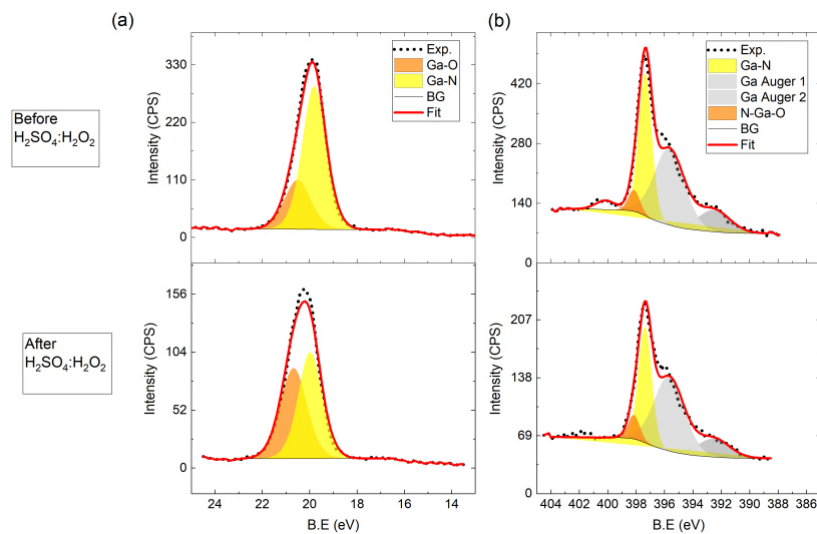
Figure 86. Evolution of (a) the Ga 3d spectra and (b) the N 1s spectra after 40 cycles of \text{H}_2\text{SO}_4:\text{H}_2\text{O}_2 mixture/ deionised water
