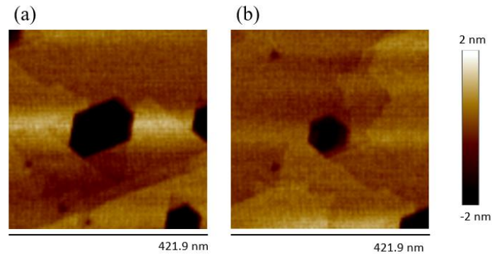
Figure 99. AFM images of (a) overlapping dislocations and (b) a single dislocation of the surface of an as-grown sample after 60 minutes in \text{H}_3\text{PO}_4
