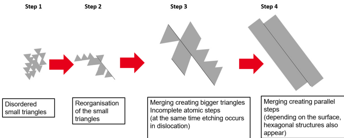
Figure 100. Evolution of the GaN surface for different durations in \text{H}_3\text{PO}_4 . The black line is a visual guide to delimit the atomic steps
