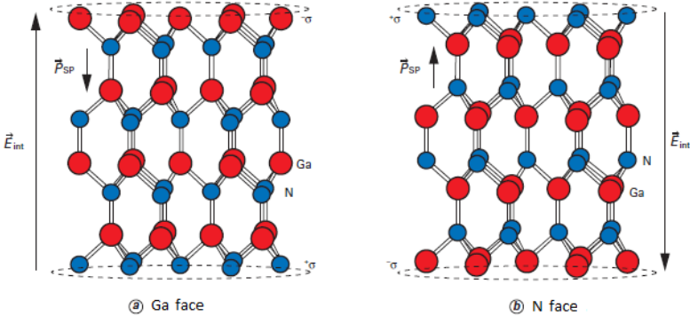
Figure 3. Spontaneous polarisation and charge distribution within the wurtzite GaN structure [10]
