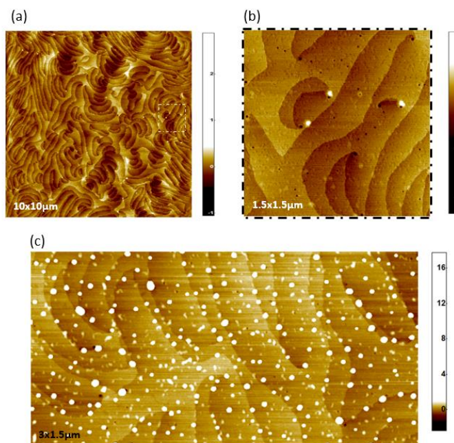
Figure 91. Evolution of the white dots after \text{H}_2\text{SO}_4\text{:H}_2\text{O}_2 treatments, (a) one month after the treatment (b) a zoom image of (a) showing the white dots near dislocations and (c) the evolution of the white dots 3 months after the treatments
