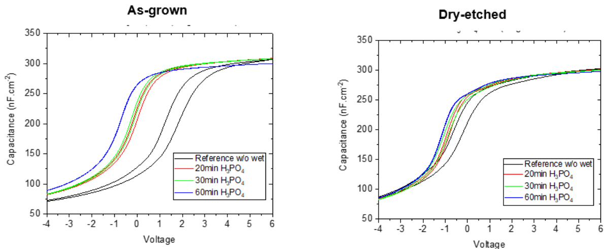
Figure 105. C-V curves before and after 20, 30 and 60 minutes in H_3PO_4 for as-grown (left) and dry-etched GaN (right)
