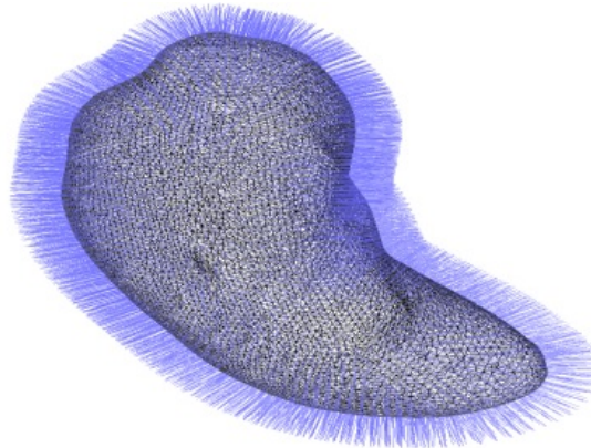
Figure 3.5: Uterus mesh; the blue lines indicate the normal of each dipole.
