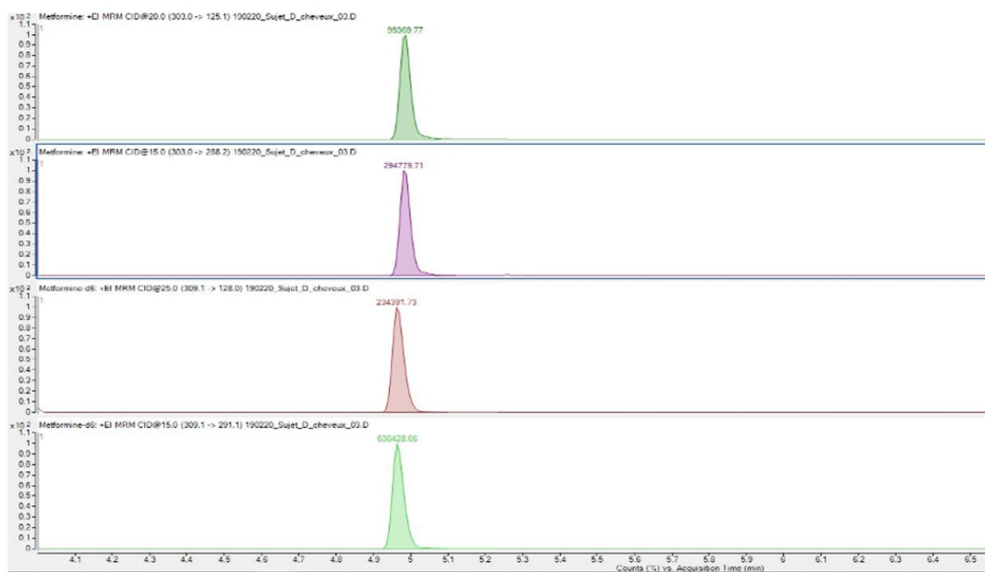
FIGURE 1 Chromatogram of subject's hair on daily treatment, 0–2 cm (from top to the bottom: 2 transitions of metformin and 2 transitions for IS metformin-d6). Concentration was 0.3 ng/mg [Colour figure can be viewed at wileyonlinelibrary.com ]
