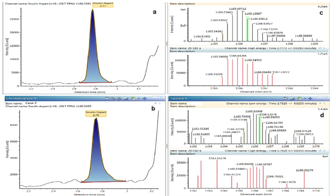
Figure 3. (a, b) Extracted chromatograms for aspart insulin from mother and daughter blood specimens (top: mother, bottom: daughter). (c, d) Spectra from 5-fold charged ions of aspart insulin from mother and daughter blood specimens (top: mother, bottom: daughter). Concentrations were, from top to the bottom, 5.7 and 2.4 ng/mL.
