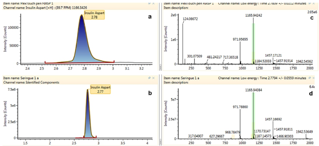
Figure 2. (a, b) Extracted chromatograms for aspart insulin from the pen and syringe solutions (top: pen, bottom: syringe). (c, d) Spectra from 5-fold charged ions of aspart insulin in the pen and syringe solutions (top: pen, bottom: syringe).
