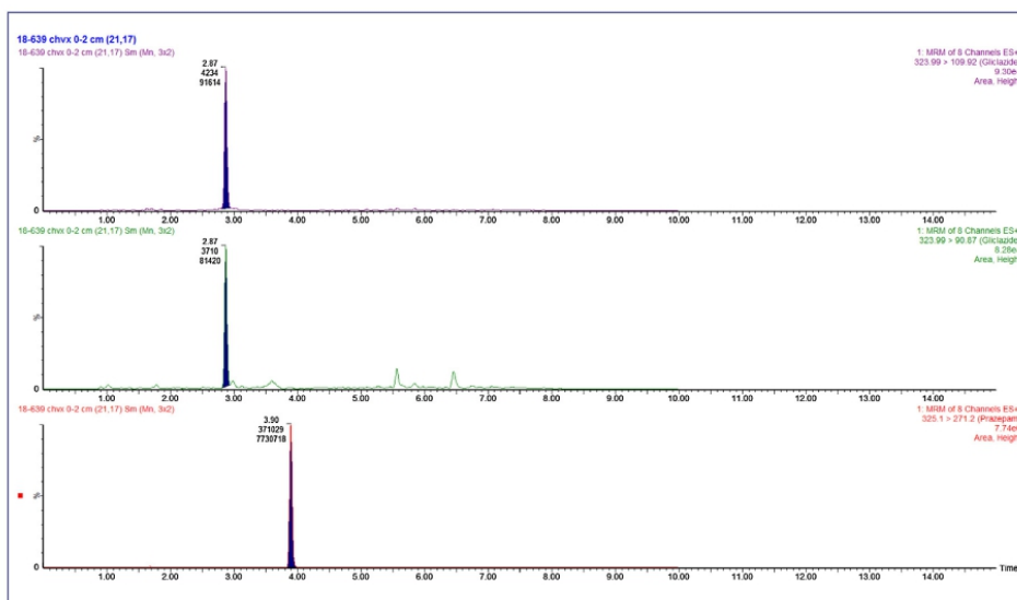
Figure 3. Chromatogram obtained after extraction of the 0 to 2 cm proximal hair segment of the victim. Gliclazide concentration was 7 pg/mg. From top to bottom: 2 transitions for gliclazide and 1 transition for prazepam (IS).
