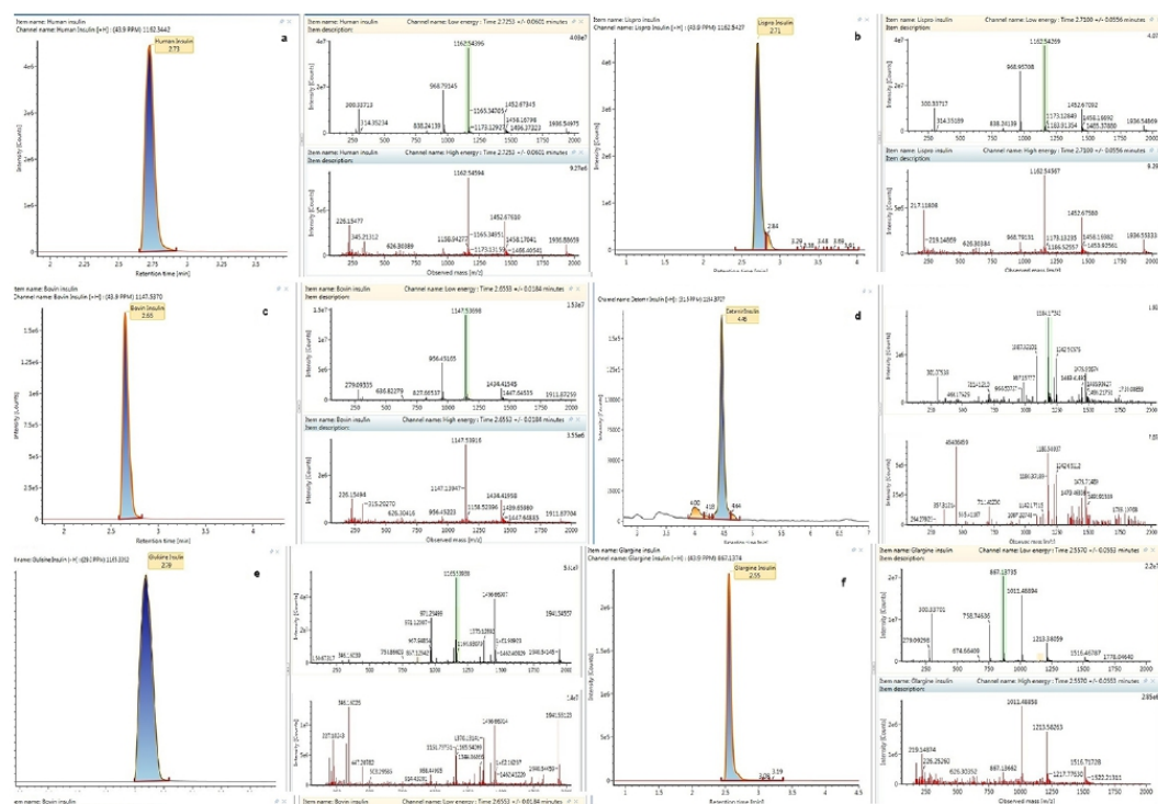
Figure 1. Spectral data information for insulin analogs by liquid chromatography coupled to high-resolution mass spectrometry (LC-HRMS). (a) Human insulin: m/z [M + 5H]^{5+} 1162.54396; (b) lispro insulin: m/z [M + 5H]^{5+} 1162.54265; (c) bovine insulin: m/z [M + 5H]^{5+} 1147.53698; (d) detemir insulin: m/z [M + 5H]^{5+} 1184.17242; (e) glulisine insulin: m/z [M + 5H]^{5+} 1165.53988; (f) glargine insulin: m/z [M + 7H]^{7+} 867.13735.
