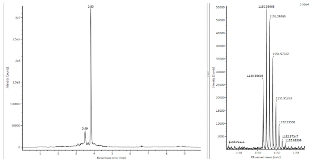
Figure 2. Extracted chromatogram and spectra information for insulin glargine metabolite M1 (21 A -Gly-insulin). M1 : m/z [M+5]^+ 1150.899969.
