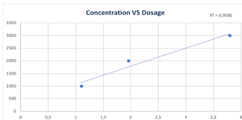
FIGURE 3 Concentration of metformin in dark hair versus daily dosage ( n = 3 ) [Colour figure can be viewed at wileyonlinelibrary.com ]
