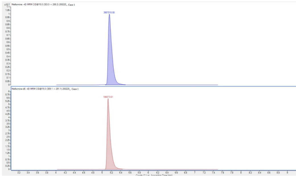
Fig. 1. Chromatogram of Subject's 1 hair, 0–2 cm (from top to the bottom: 1 transition of metformin and 1 transition for IS metformin-d6). Concentration was 28.3 ng/mg.
