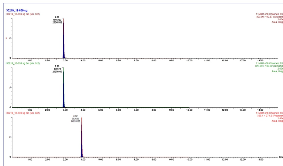
Figure 1. Chromatogram obtained after extraction of the femoral blood of the victim. Gliclazide concentration was 2.20 mg/L. From top to bottom: 2 transitions for gliclazide and 1 transition for prazepam (IS).
