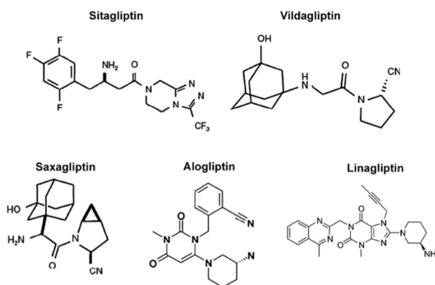
Figure 6. Structures chimiques des gliptines [40]
