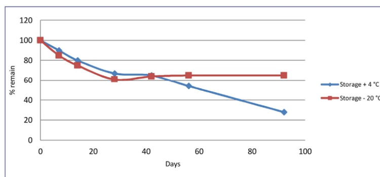
Figure 2. Percentage of concentration remaining from the initial 10 mg/L of gliclazide when stored at +4 °C and -20 °C for 3 months.
