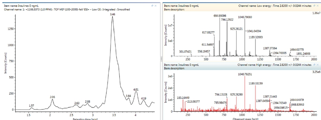
Figure 4. Chromatogram obtained after extraction of blank blood sample.
