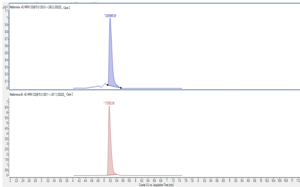
Fig. 2. Chromatogram of Subject's 2 hair (from top to the bottom: 1 transition of metformin and 1 transition for IS metformin-d6). Concentration was 22.5 ng/mg.
