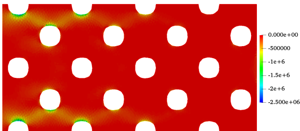
(a) Shape derivative j(\Omega) (2.12) extended to \Omega
