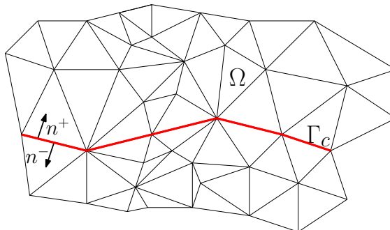
Figure 3.4: Coincident boundary mesh of \Gamma^h , representing the contact surface \Gamma_c
