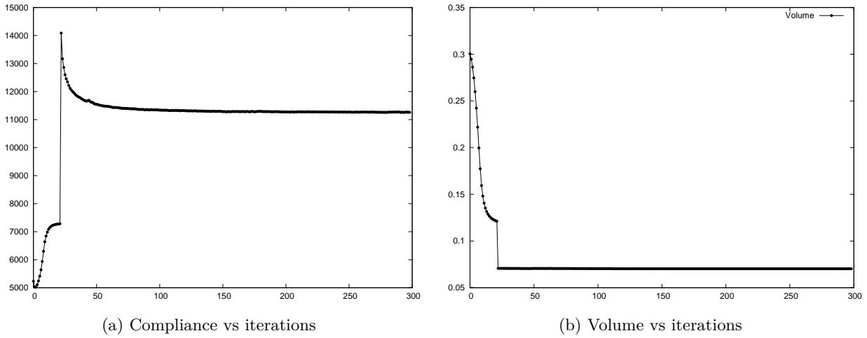
Figure 7.5: Convergence history for the shape in Fig.7.4c
