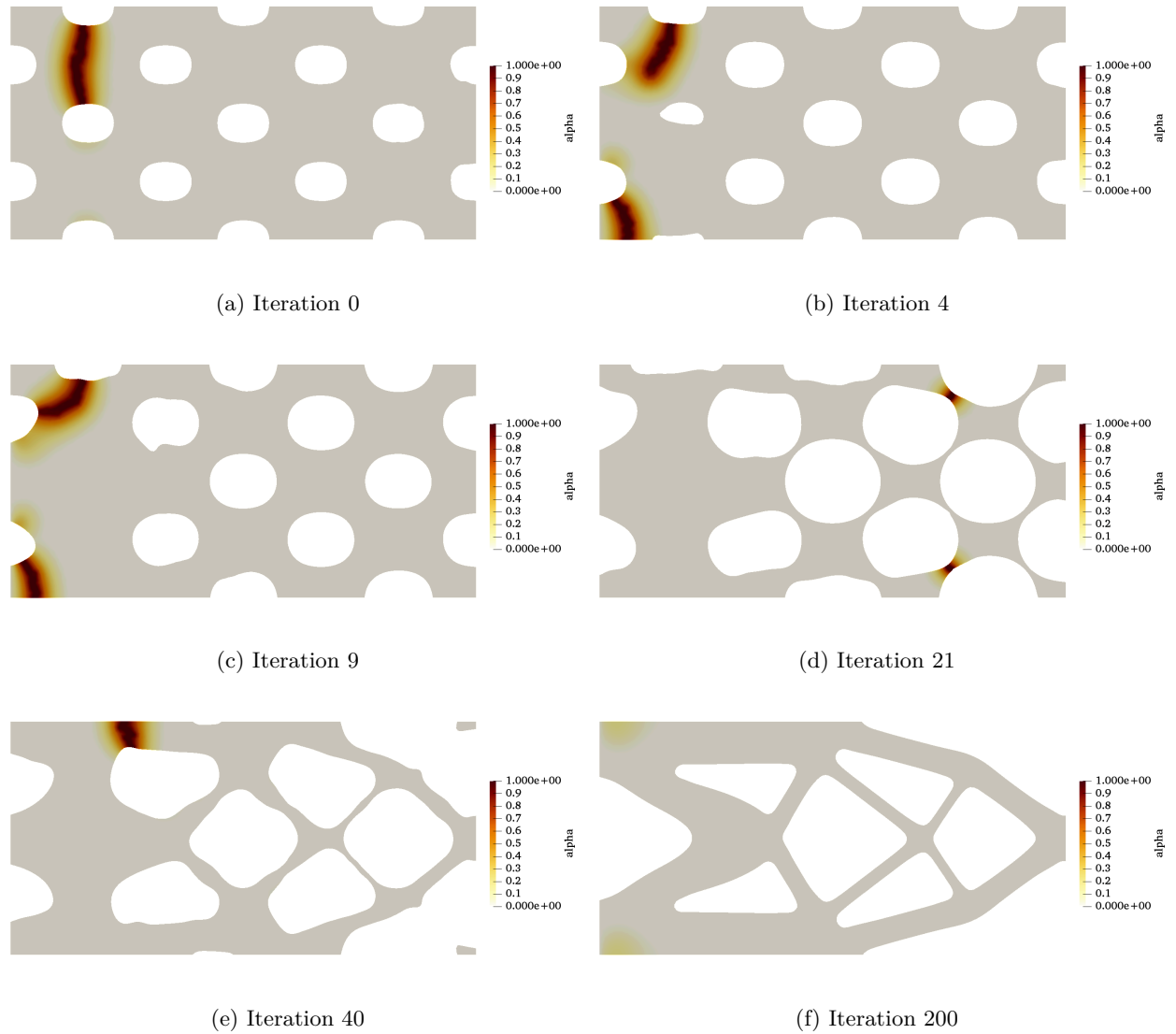
Figure 6.7: damage variable \alpha at the final time plotted for several optimization iterations for the shape in Fig.6.5c
