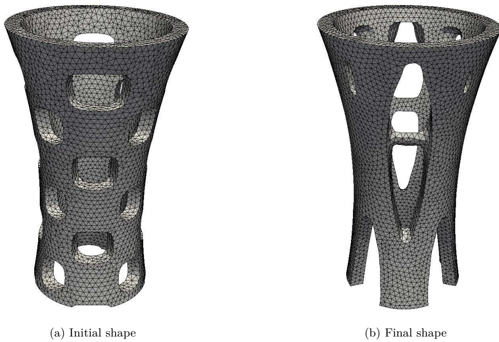
Figure 2.17: Meshed column, minimization of compliance 2.3
