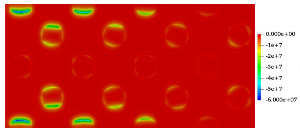
(b) Regularized shape derivative dj_\alpha(\Omega) (using (2.23))
