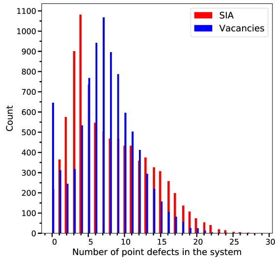
Figure 3.4: The analysis of the distribution of randomly generated point defects in the random database . This database is derived from the ARTn database only using the supercells of volume (10a_0)^3 and (12a_0)^3 by random creation of Frenkel pairs. The plot emphasizes the occurrences in the entire random database of number of SIAs and vacancies in the same supercell. The random database contains 9016 configurations.
