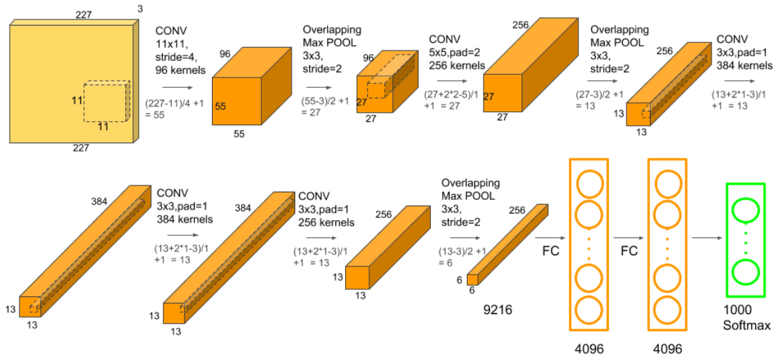
Figure 1.1: The architecture of the AlexNet CNN [Krizhevsky et al., 2012]. Convolution operations are represented by an arrow with CONV, the spatial size of the convolution, the stride of the convolution, and the number of convolutional kernels (i.e., filters). Convolutions are followed by a ReLU non-linearity which is not represented in the figure. Max-pooling operations are represented by an arrow with Max POOL, the spatial size of the region, and the stride. Fully-connected operators linear operators are represented by an arrow with FC and are followed by a ReLU non-linearity.
