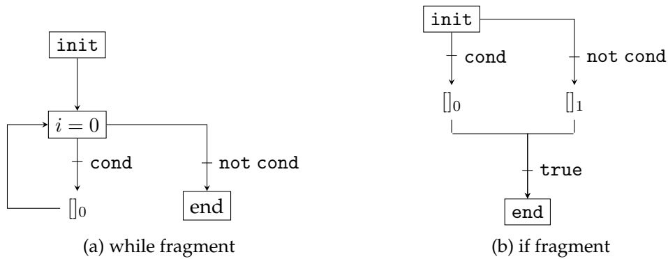
Figure 2.3: Program Fragments
