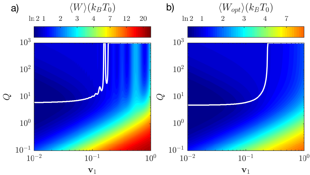
Figure Cl.1 – a) Energetic consumption of a [RESET] operation , computed from the model detailed and experimentally validated in chapter 4 (same as Fig. 4.9). The average work required to erase 1-bit of information is displayed as a function of the driving speed \mathbf{v}_1 = Z_1/(\tau\omega_0) and the memory quality factor Q . The optimal damping is emphasized in white: it results from a balance between the price of the compression warming prevailing when Q is high (but bounded by the adiabatic limit), and the dissipation cost prevailing when Q is low. Let us point out that as the operation is logically irreversible the energetic consumption is bounded by the Landauer’s fundamental lower limit. b) Energetic consumption of an optimal [RESET] operation computed from the model adapted to the optimal protocol, and validated by simulation results (same as Fig. 4.13b)). Applying optimal translational drivings substantially reduces the erasure cost for all damping regimes and driving speeds as highlighted by the common color scale used for a) and b). Similarly to the observations in a), the optimal quality factor (white line) is around Q = 8 at low speed, and increases strongly for fast operations.
