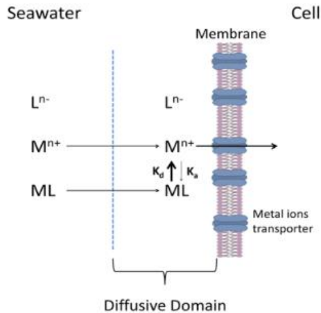
Figure 1.6: Internalization of free ions through the cell membrane of a phytoplankton, where M represents a metallic element and L a ligand (Baeyens et al., 2018a).
