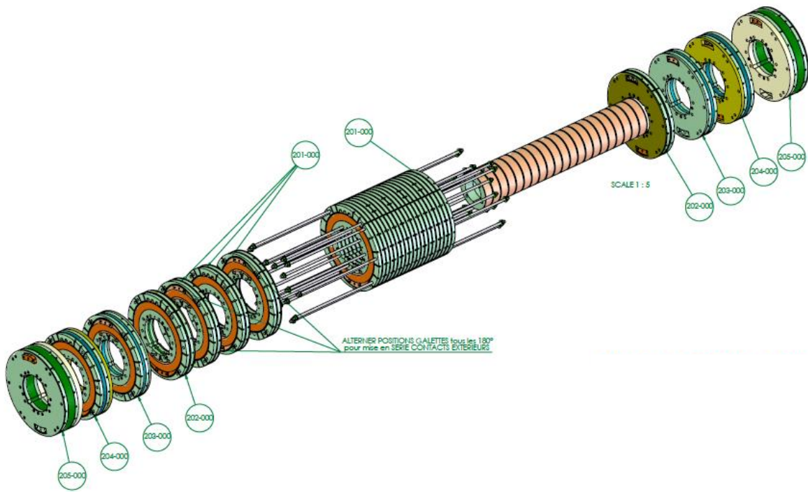
Fig. 88. Schematic view of the solenoid assembly.
