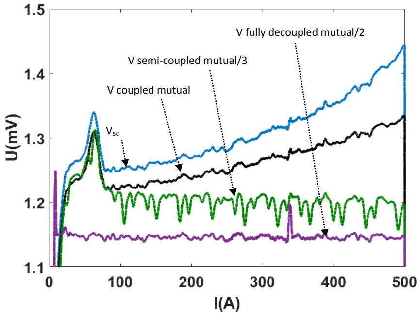
Fig. 66. Voltages from the REBCO pancake ( V_{sc} , light blue) and the 3 pick-up coils (V coupled mutual in black, V semi-coupled mutual/3 in green and V fully decoupled mutual/2 in purple) for the first current ramp up to 500 A.
