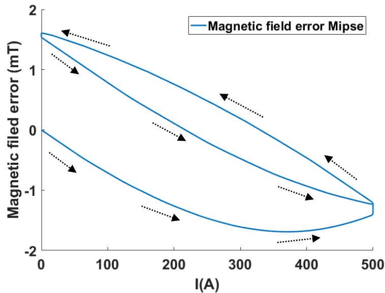
Fig. 64. Magnetic field error from Mipse corresponding to screening current field at the coil center.
