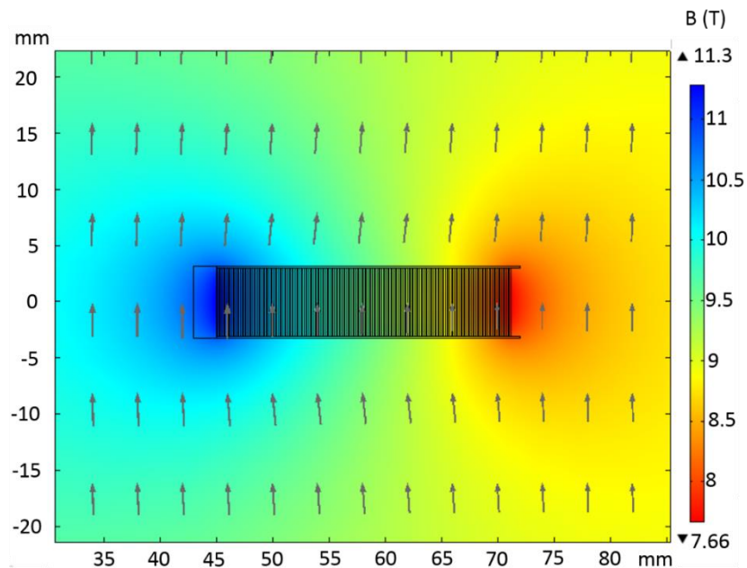
Fig. 136. 2D axisymmetric modeling of the magnetic field generated by the pancake at a current of 370 A under 9 T of magnetic background field. The differences in thickness between the turns as well as the periodic structures of the pancake turns that can be visualized are due to the graphic resolution of the image.
