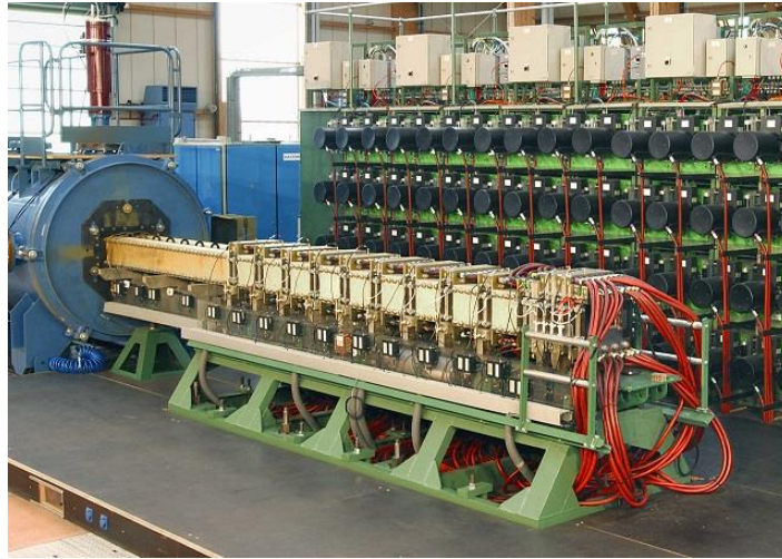
Fig. 82. Pegasus 10 MJ launcher (from ISL).
