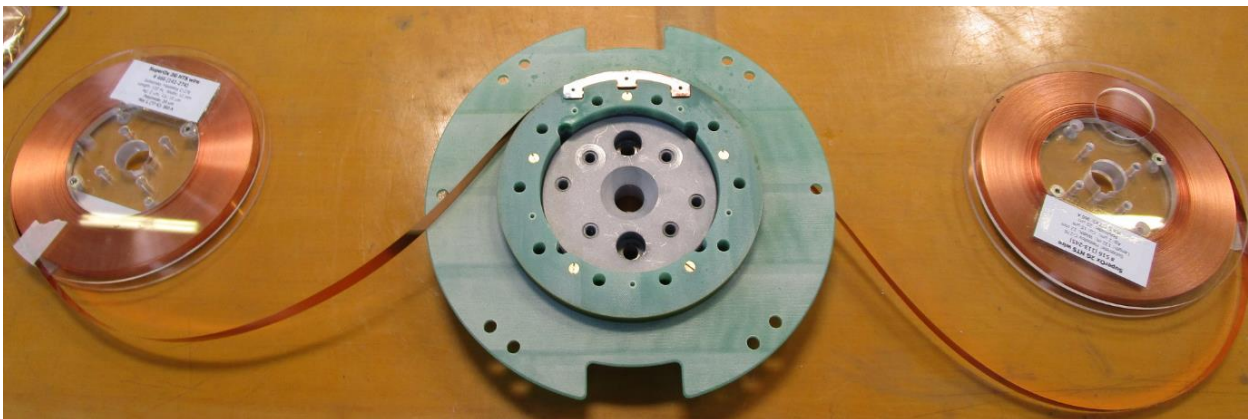
Fig. 91. Tooling and soldering of the inner contacts.
