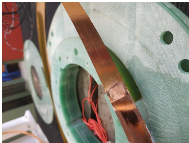
Fig. 113. Pinched conductor at the exit of the inner contact.
