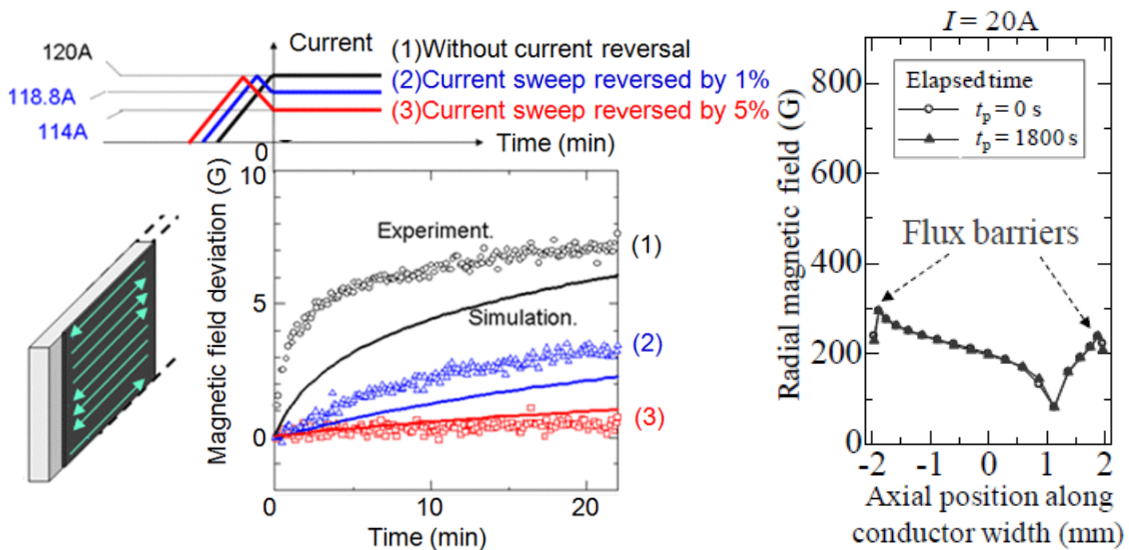
Fig. 24. To the left: (1) Magnetic field drift without current overshoot, (2) Magnetic field drift with a current overshoot of 1%, (3) Magnetic field drift with a current overshoot of 5% [27]. To the right: Magnetic field distribution at 20 A in the superconductor in the innermost layer of the upper coil end obtained by numerical simulation [28].
