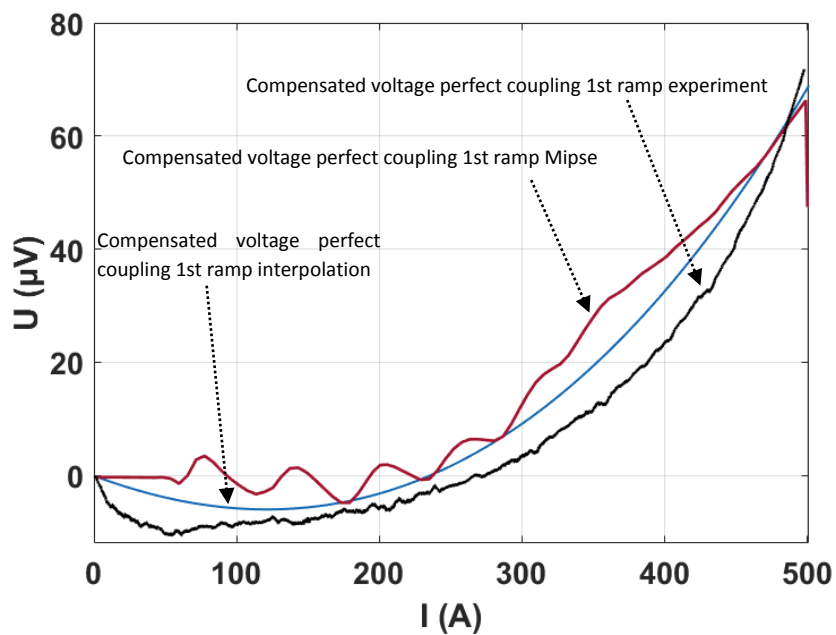
Fig. 71. Compensated experimental voltage with the “perfect” coupling for the first current ramp up to 500 A compared to the modelling results. Experimental curve in black, Mipse curve in red and the interpolation in blue.
