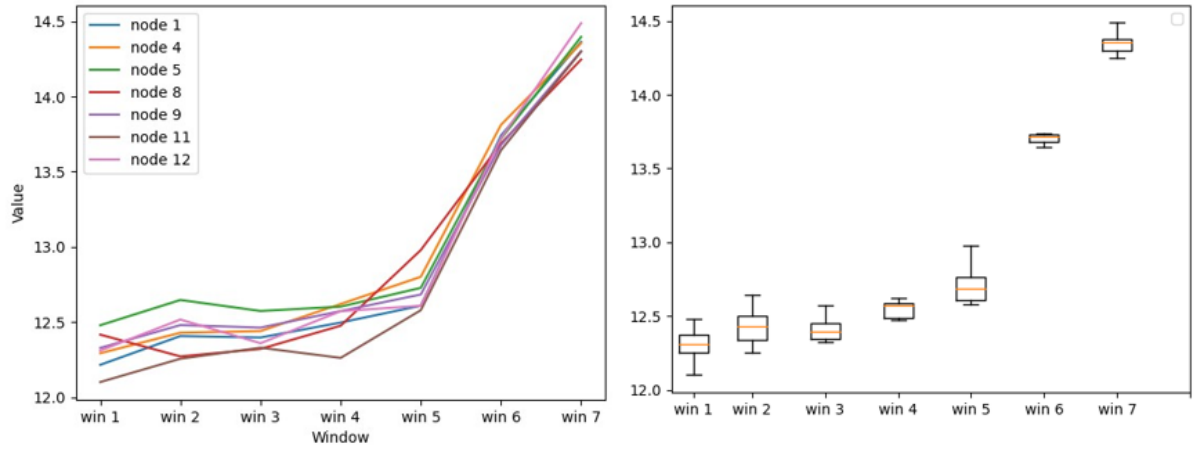
Figure A.16 Analyses of each window for the methods H2(Str)
