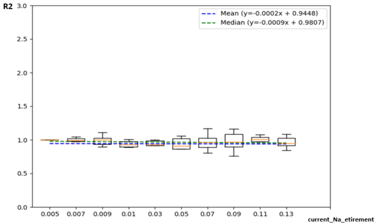
Figure B.1 Evolution of R2 function of the tissue current_Na_etirement
