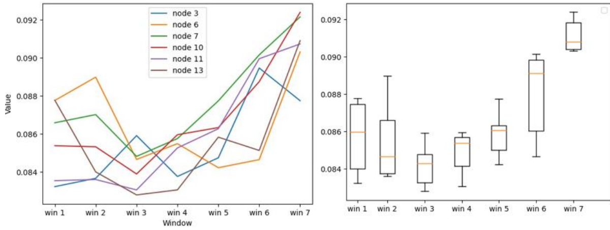
Figure A.32 Analyses of each window for the methods ICOH(PR)
