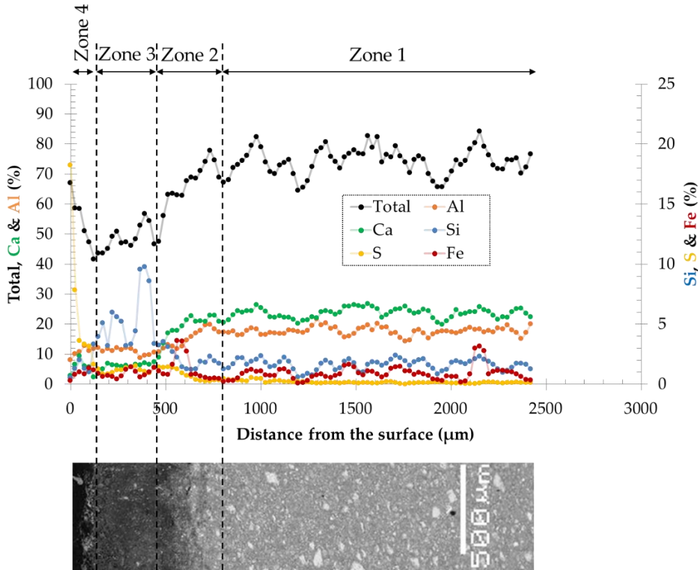
Figure V-7. Evolution of the chemical composition of the CAC material exposed to the BAC test for 3 months as a function of the distance from the initial surface of the specimen (at 0 μm) and the SEM observation of the microstructure of the cross-section in BSE mode
