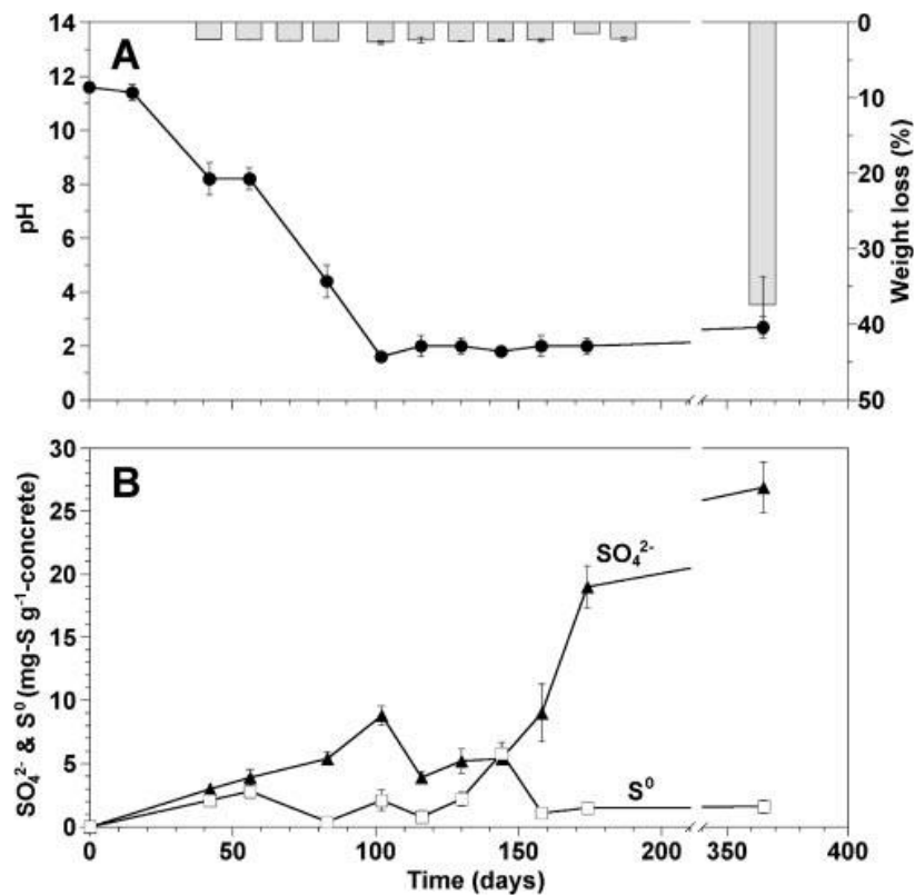
Figure I-8. (A) pH evolution and mass loss of concrete specimens exposed to sewage environments (B) \text{SO}_4^{2-} and \text{S}^0 concentrations measured on the surface of concrete specimens [42]
