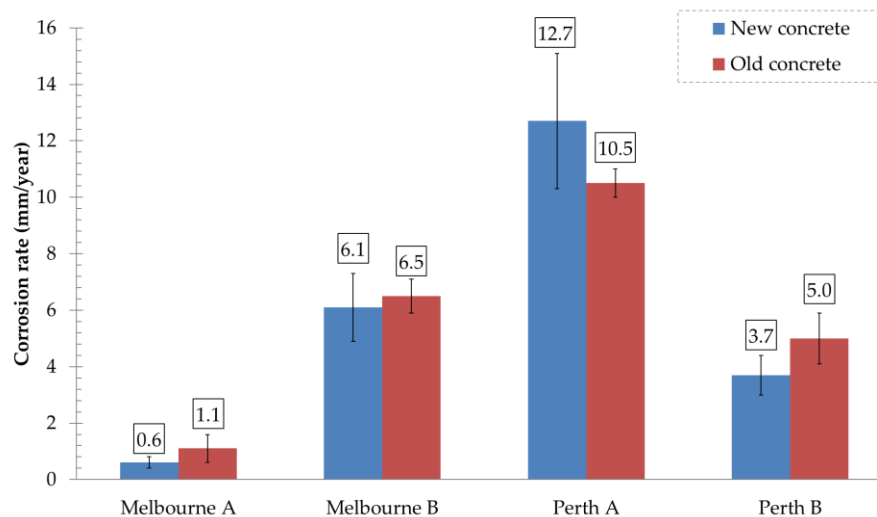
Figure I-9. Corrosion rate for new and old concrete samples exposed at Melbourne and Perth sewer systems [43]
