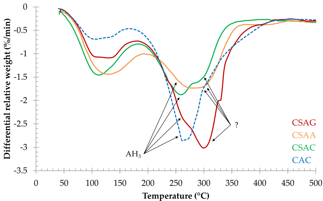
Figure V-27. DTG curves of the deteriorated zone for CAC, CSAC, CSAA and CSAG
