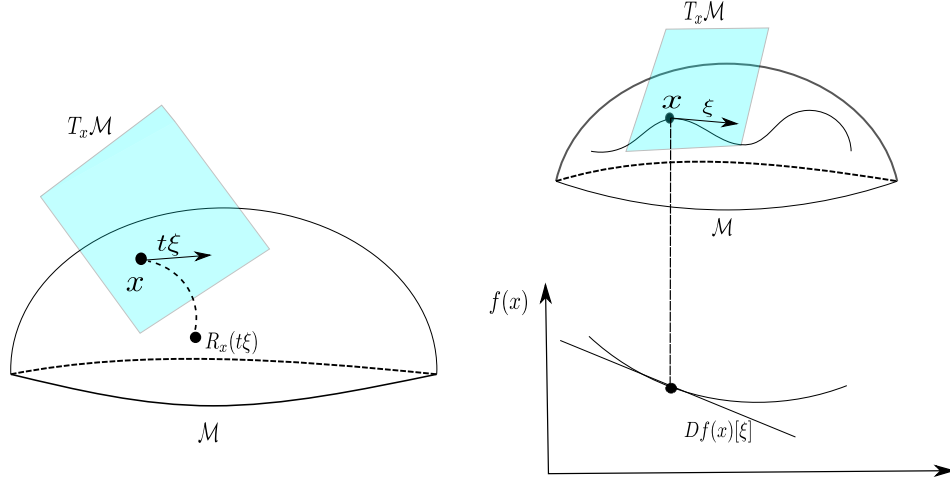
Figure 3.2 – Illustration of one step of a typical Riemannian optimization method. On the right at x a descent direction \xi which leads to a decrease in f (i.e. Df(x)[\xi] < 0 ). On the left, the new point is defined on the manifold \mathcal{M} by using a retraction operator.
